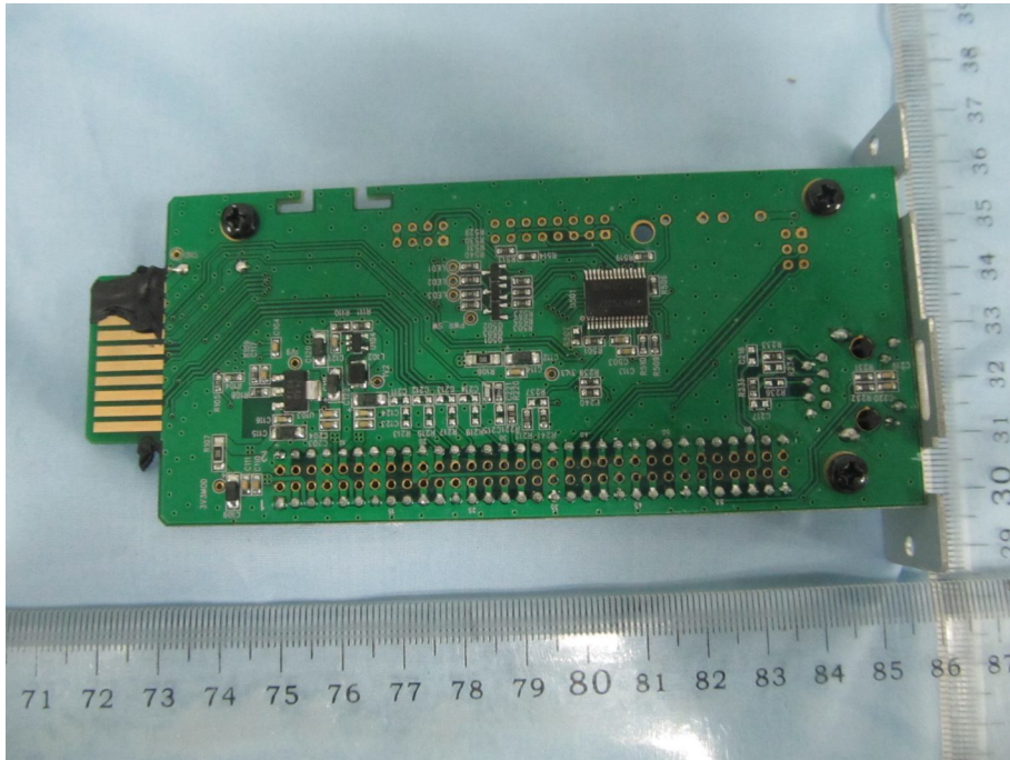
PCB of RF module
