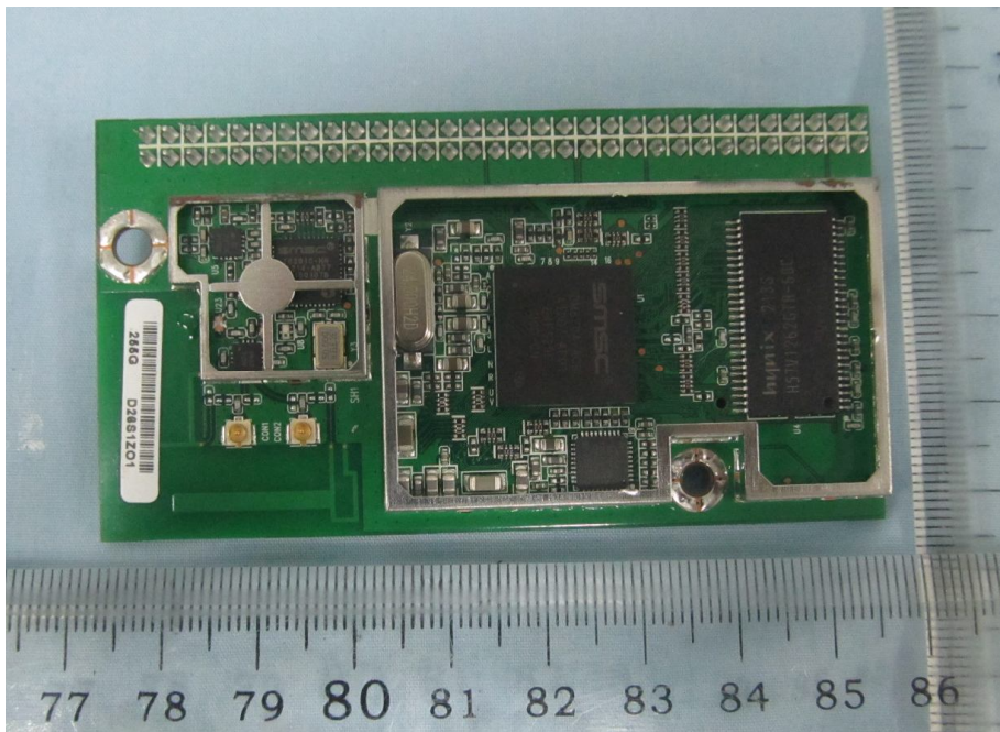
PCB of RF module
