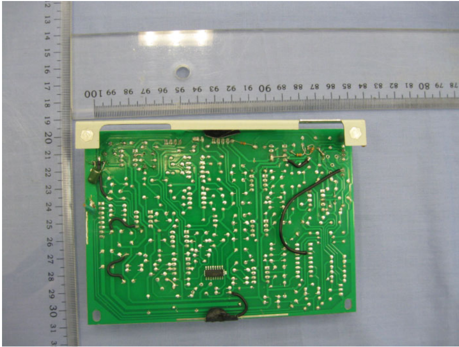
Preamplifier board
