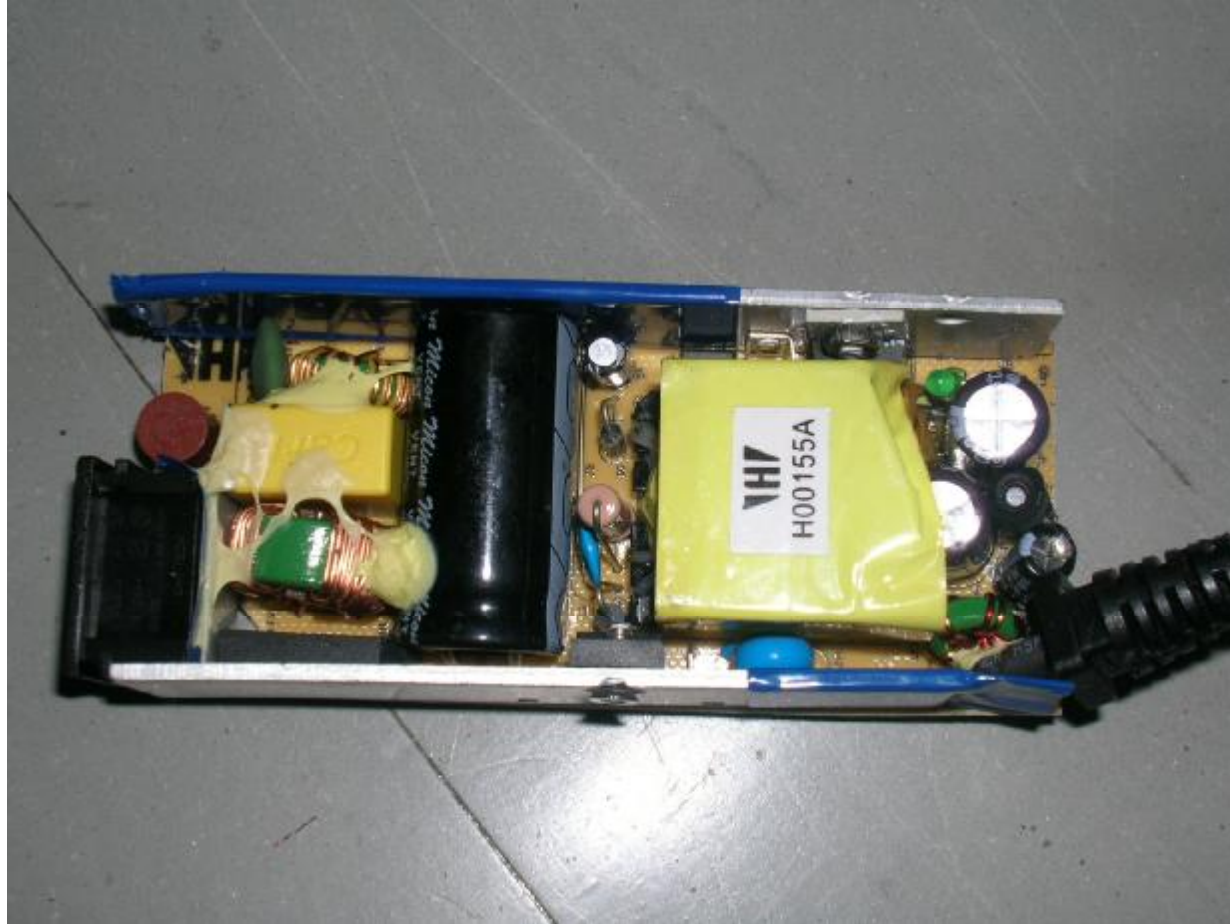
AC/DC Adapter (Component Side View)
