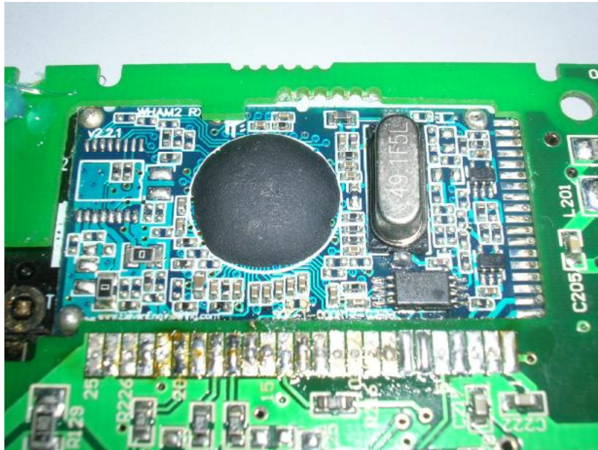
RF Module Rear View
