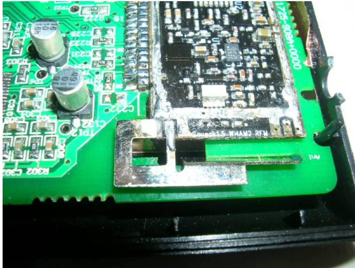
Antenna Zoom In (without shielding)
