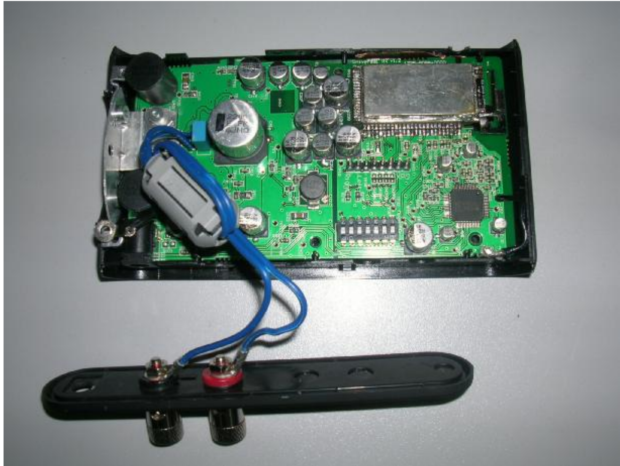
EUT (Component Side View)
