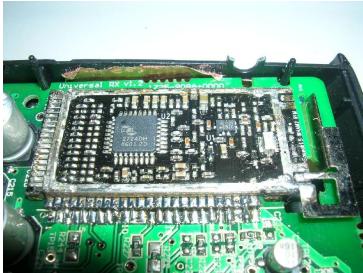
RF Module Top View (without shielding)
