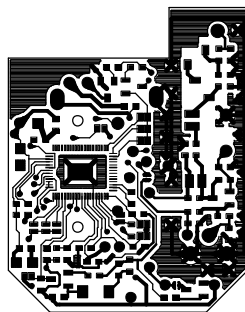
TOP COPPER
