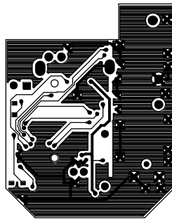
BOTTOM COPPER
