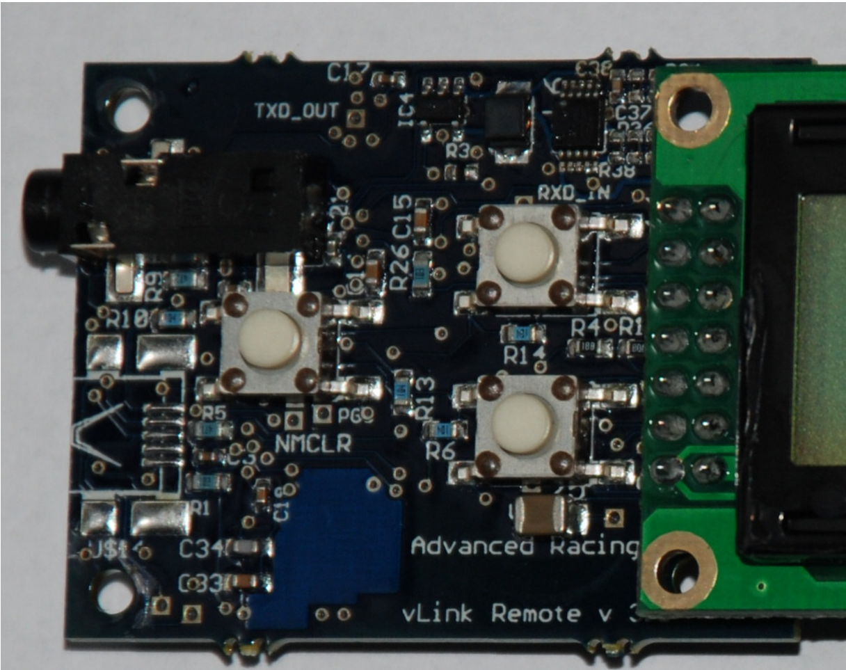
Close-up of board with radio (component side):
