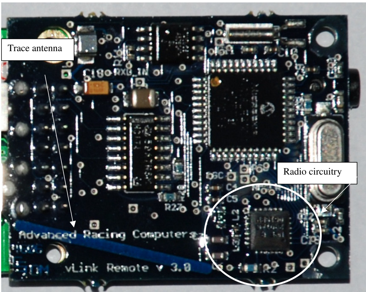
Close-up of remote board with radio circuitry (solder side):
