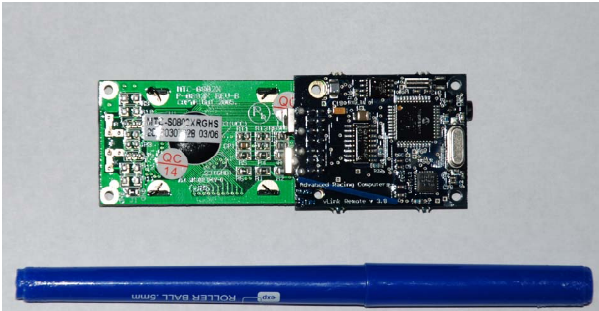
Close-up of remote board with radio circuitry (solder side):
