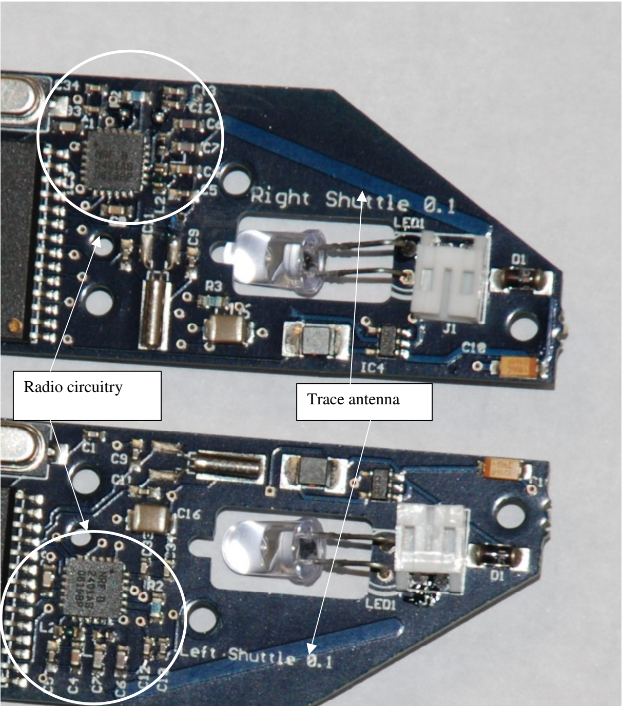
Close-up of radio on shuttle boards (component side):
