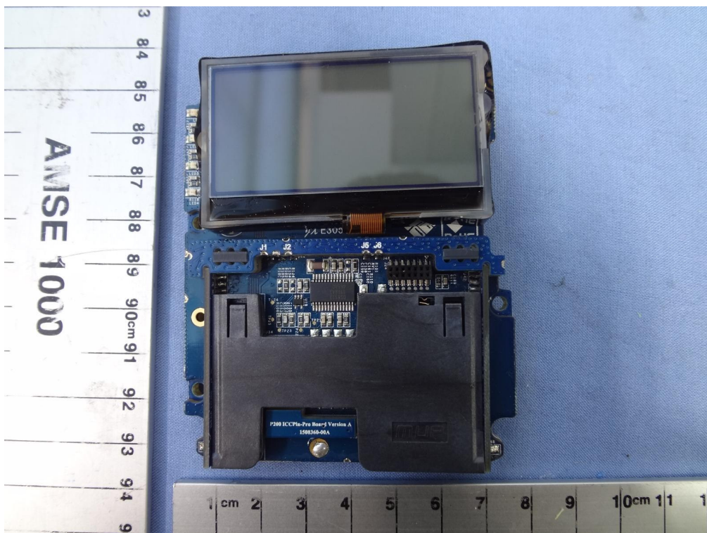
RF Board Front View
