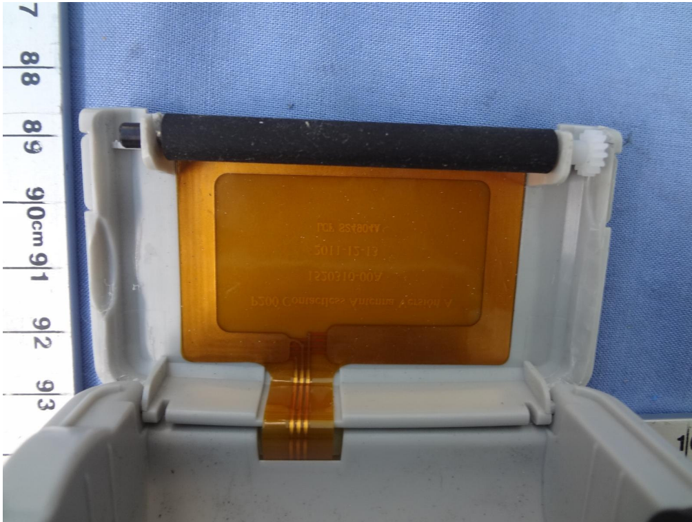
RFID 13.56 MHz LOOP Antennas
