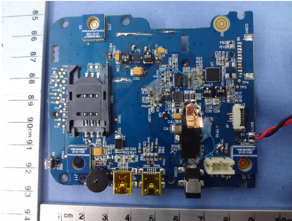
Internal of PCB Front View
