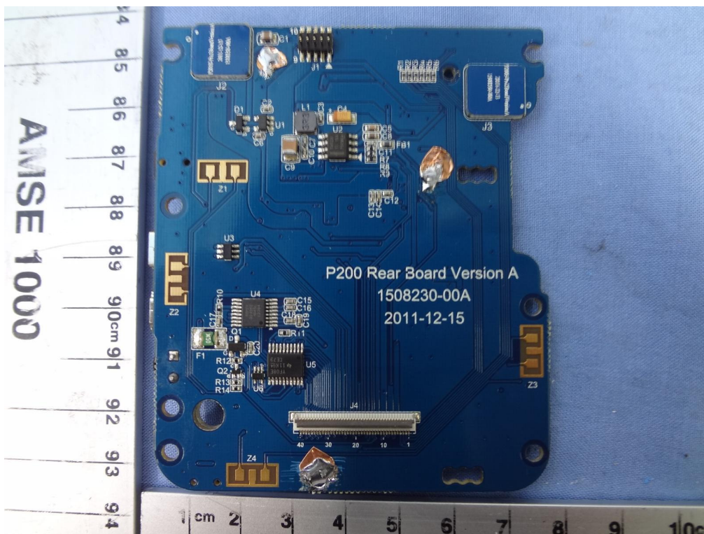
Internal of PCB Rear View
