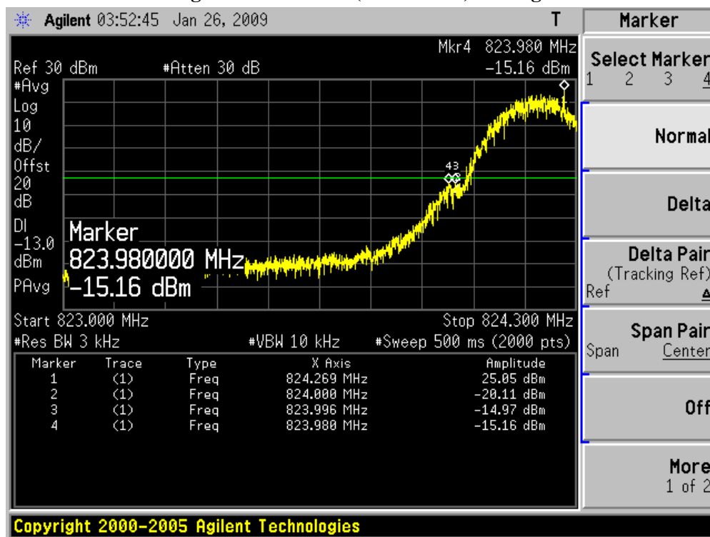
Figure Channel 128 (824.20MHz)-Average
