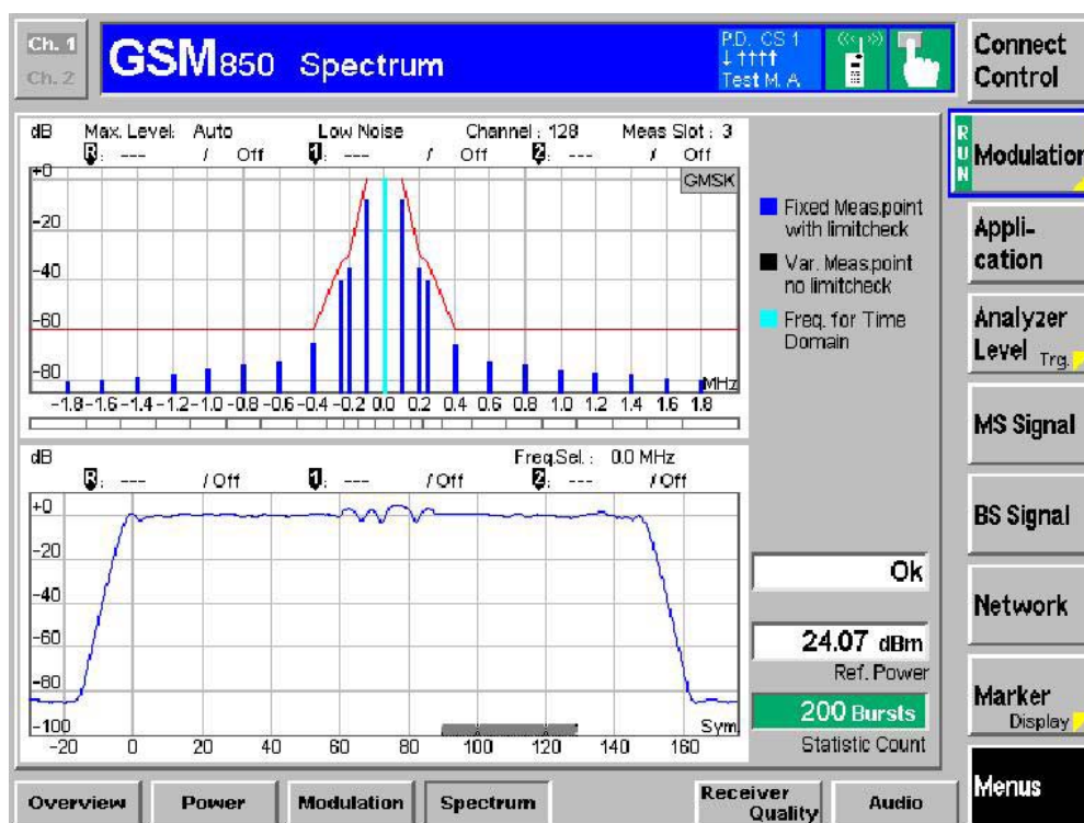
Figure (GPRS 850)
