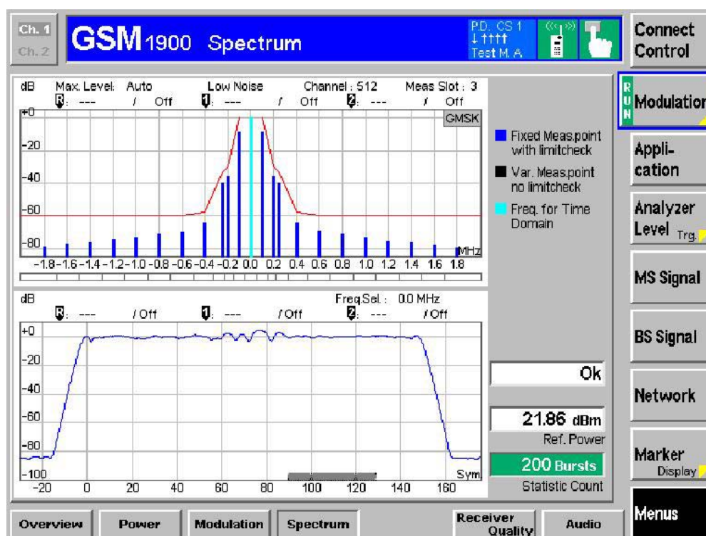
Figure (GPRS 1900)
