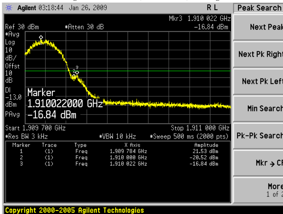
Figure Channel 810 (1909.80MHz) -Average
