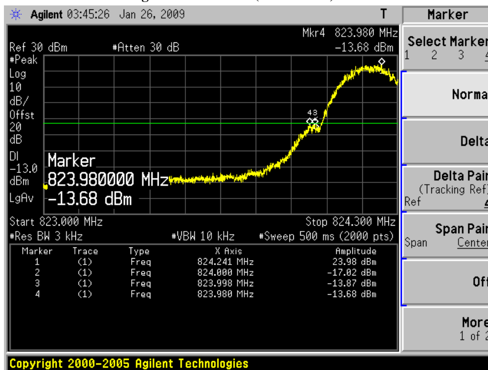
Figure Channel 128 (824.20MHz)-Peak
