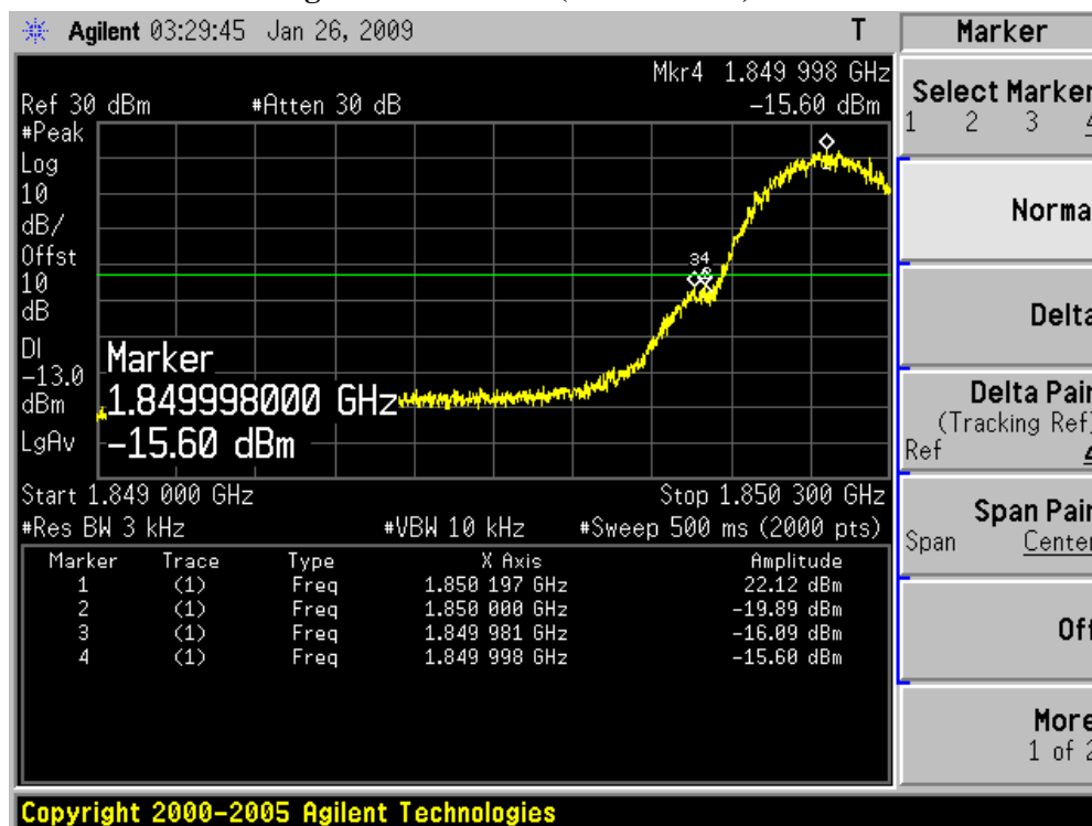
Figure Channel 512 (1850.20MHz) -Peak
