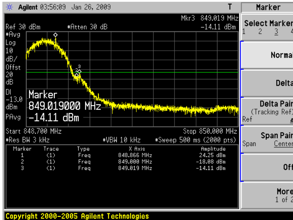
Figure Channel 251 (848.80MHz)-Average
