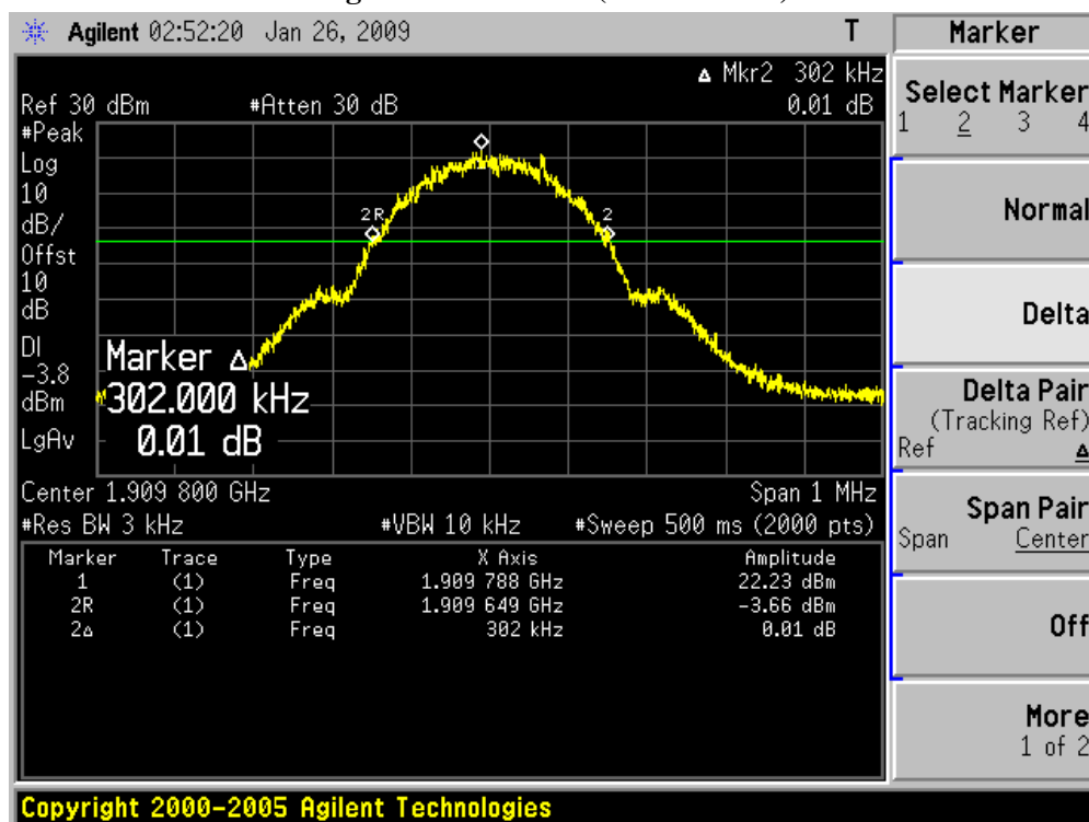
Figure Channel 810 (1909.80MHz)
