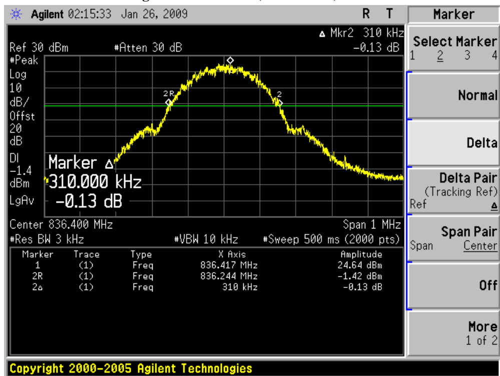
Figure Channel 189 (836.40MHz)
