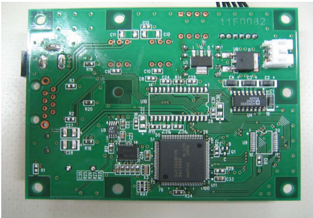
RW CONTROL Unit(Bottom)
