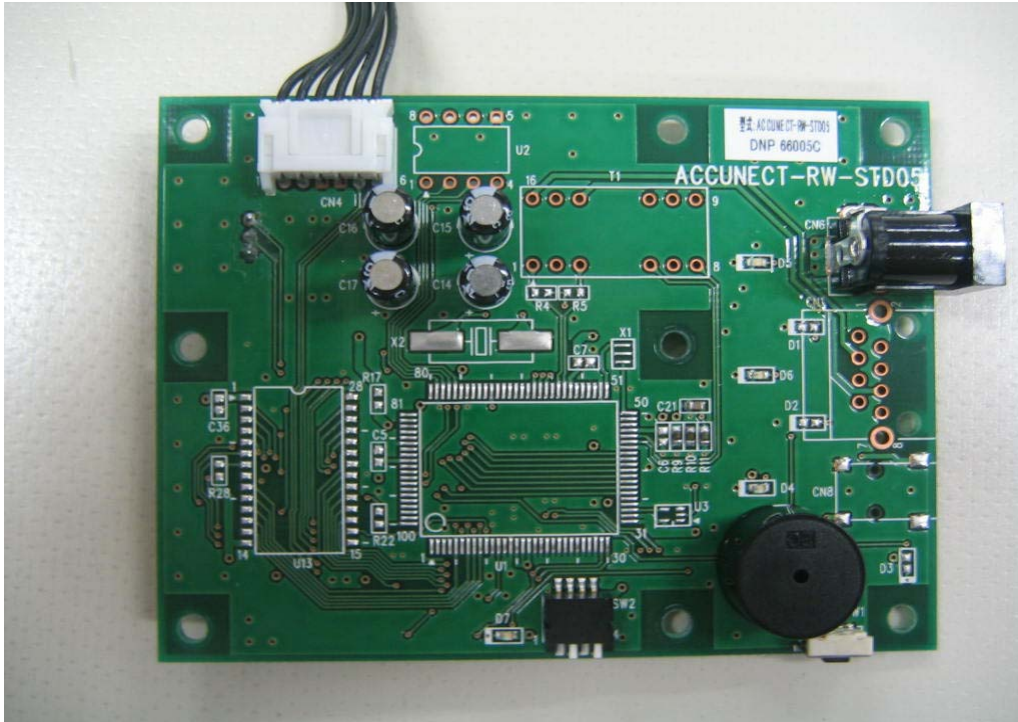
RW CONTROL Unit(Top)
