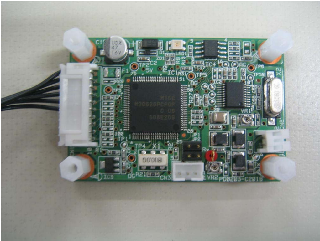
RW Module Unit (Top)
