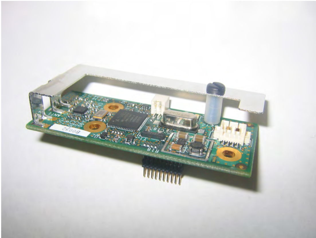
Transceiver Isometric View
