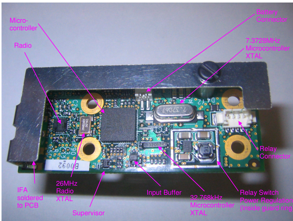
Transceiver Top View – Antenna
