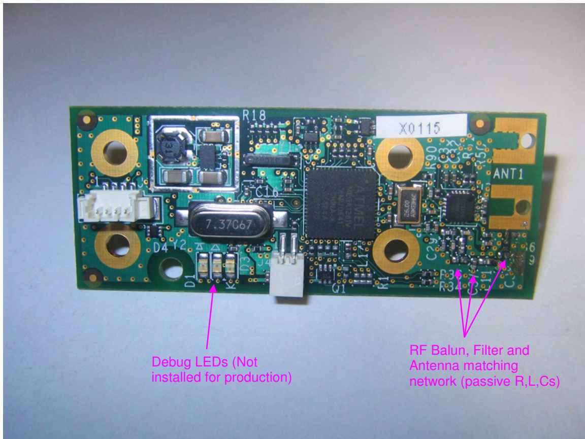
Transceiver Top View – No Antenna
