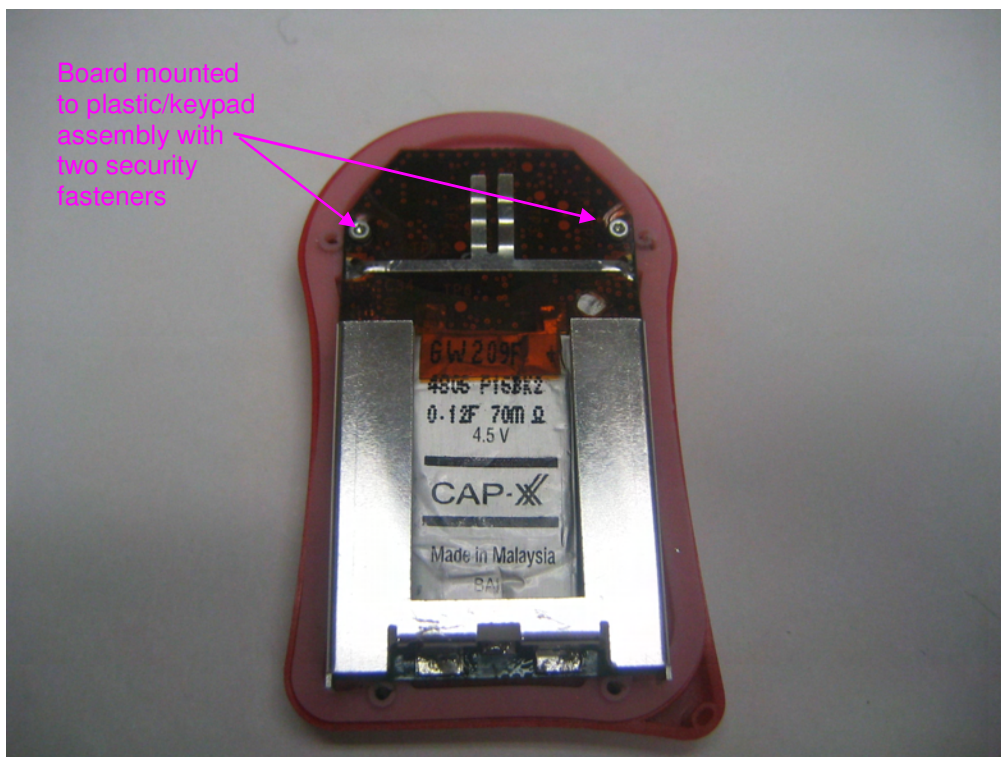
Top Half Assembly
