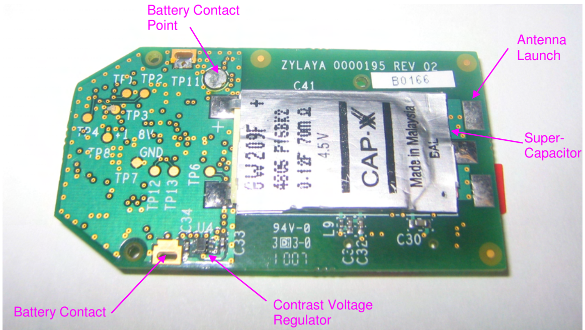
Circuit Board Assembly Bottom View
