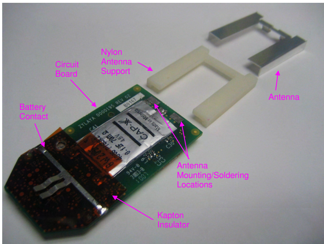
Assembly View - Exploded
