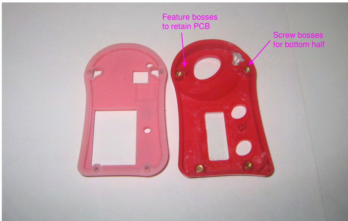
Top Plastic Housing and Rubber Keypad Bottom View
