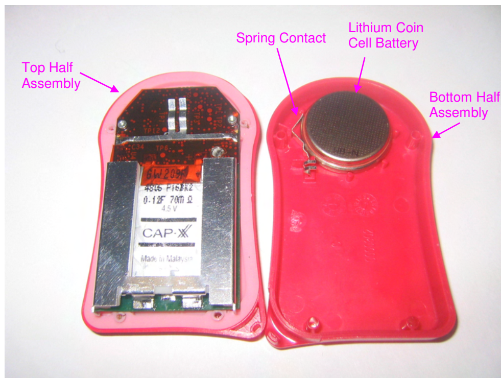
Top and Bottom Half Assembly Exploded View
