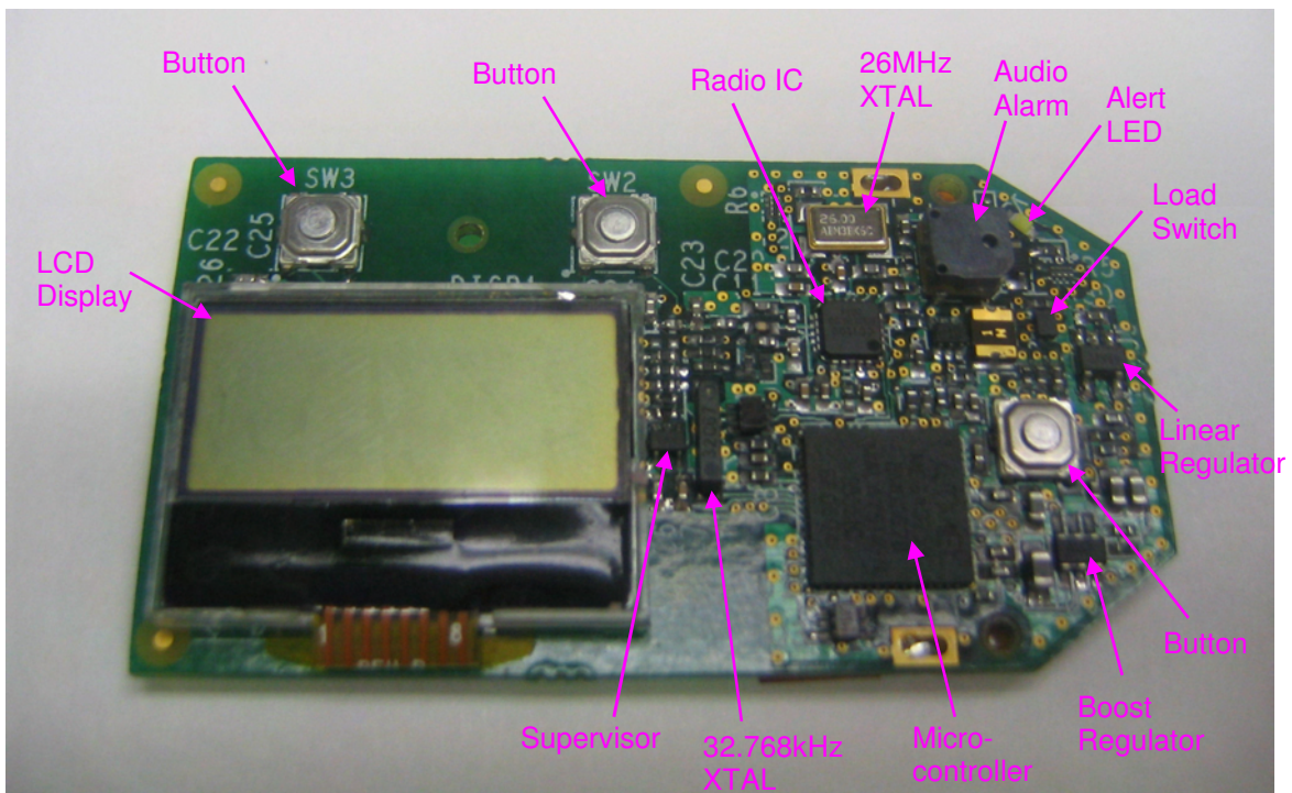
Circuit Board Assembly Top View
