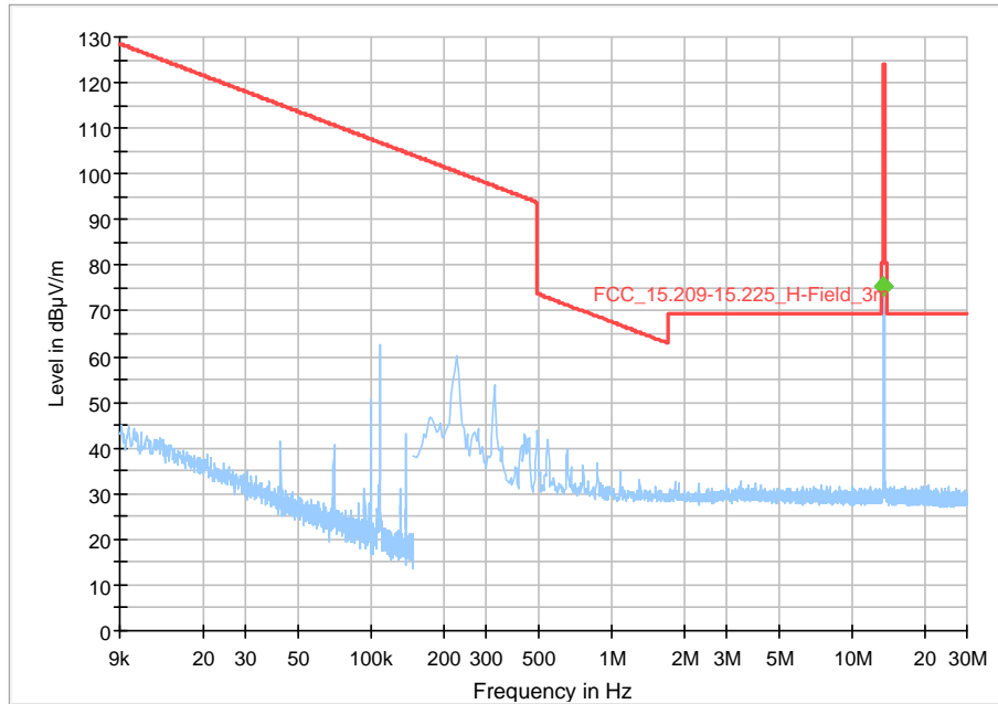
◆ Preview Result 1-PK+ Final_Result QPK ◆ FCC_15.209-15.225_H-Field_3m Final_Result AVG
