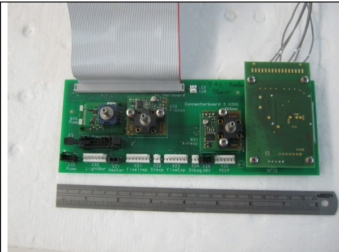
Photograph 2.3-3: Connection board with M21 connected
