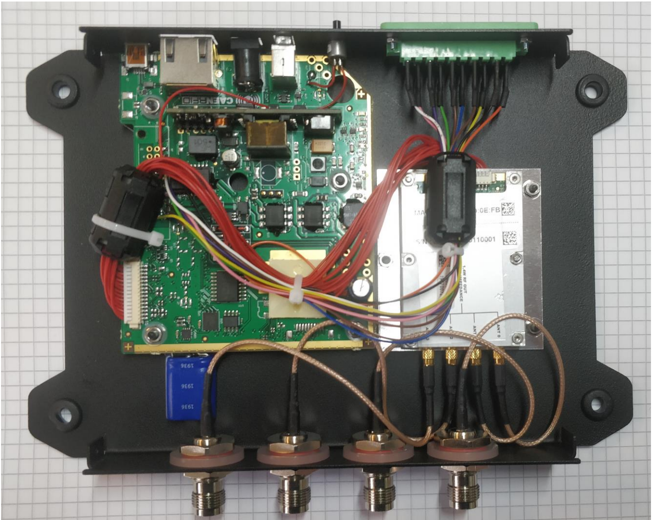
Fig. 3: Internal assembly
