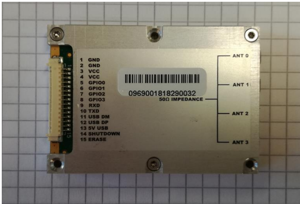
Fig. 7: RFID Module – External view - Bottom side
