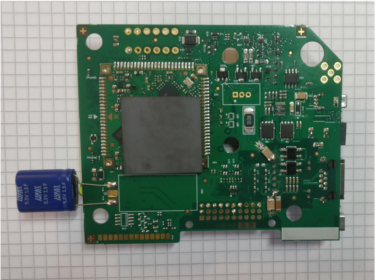
Fig. 2: Main Board - Bottom side
