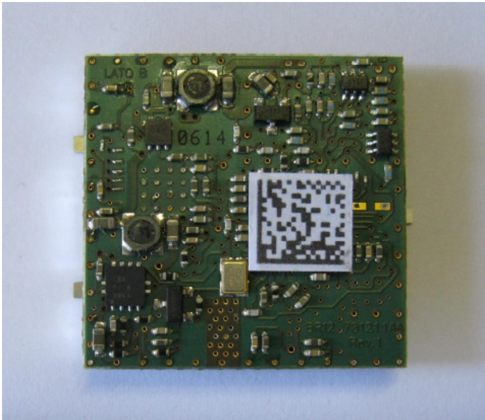
Figure 10: RFID Module - Bottom View
