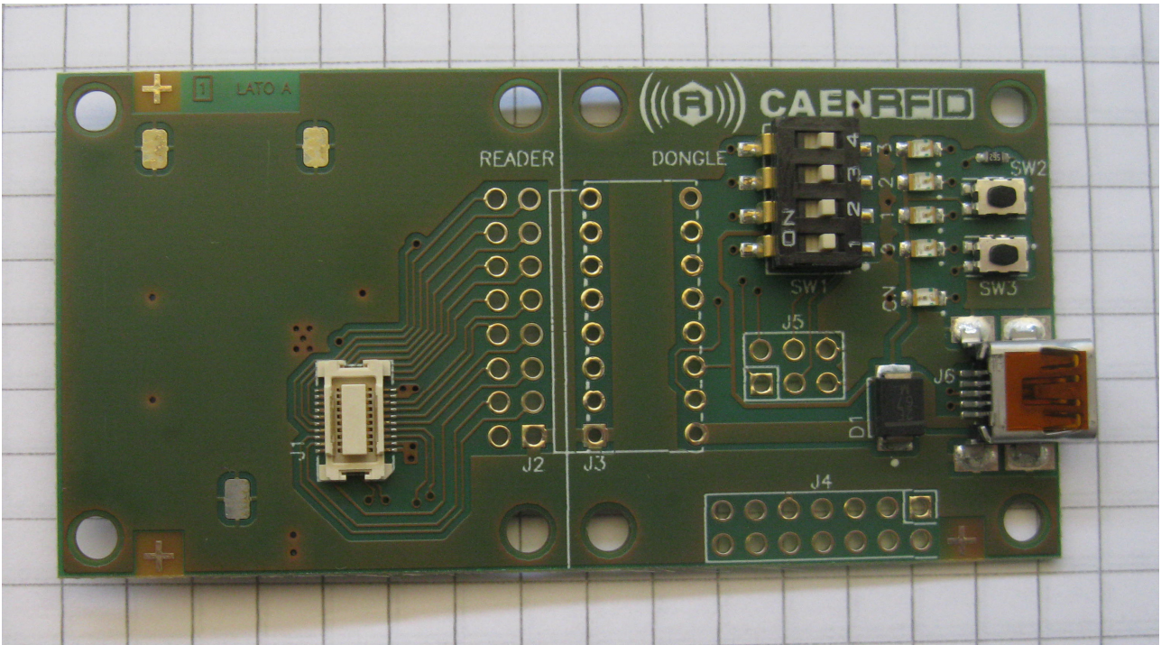
Figure 4: Interface board - Top View
