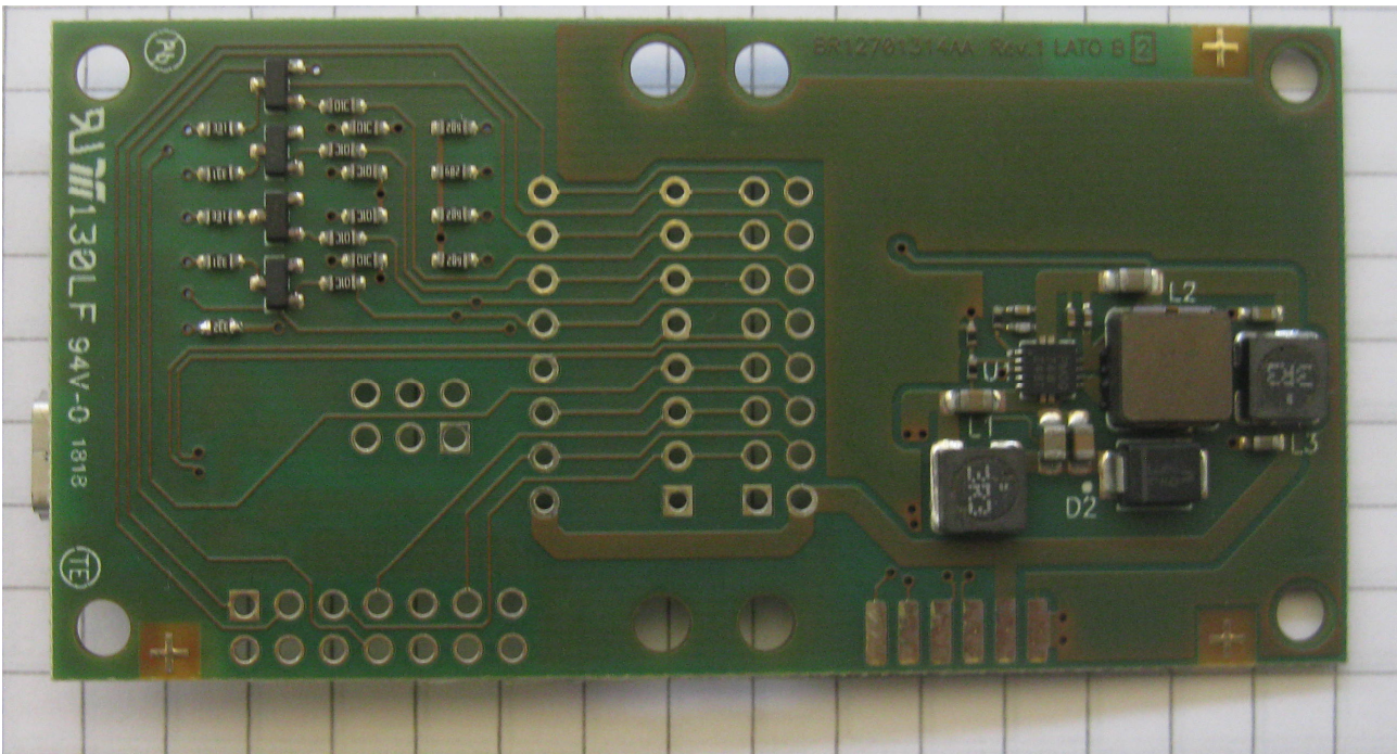
Figure 5: Interface board - Bottom View
