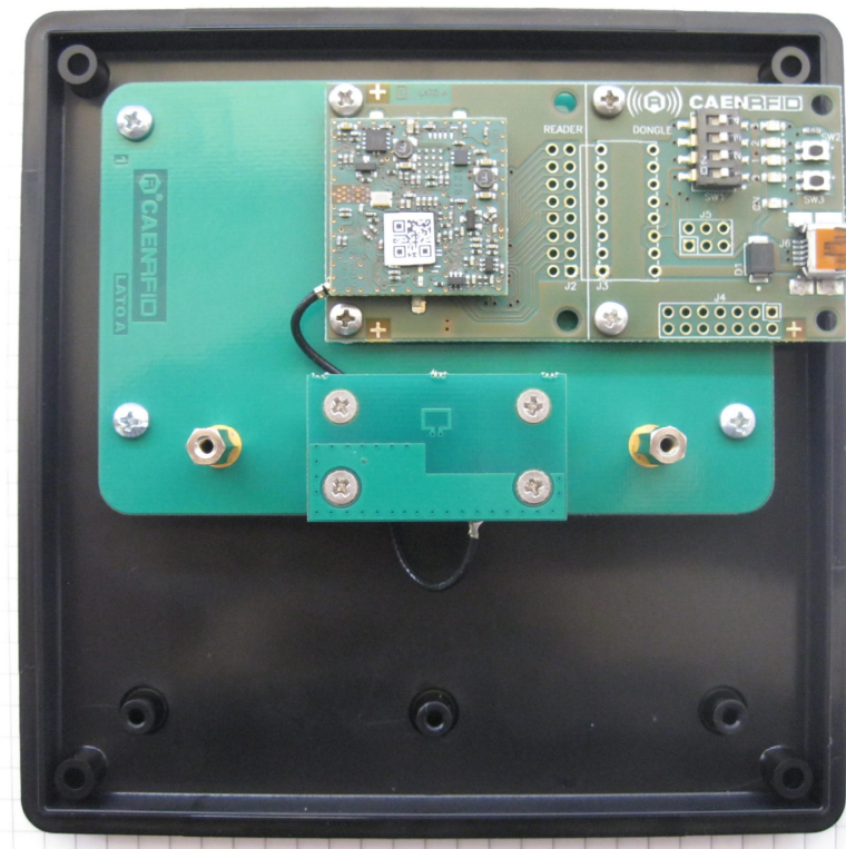
Figure 3: Internal View
