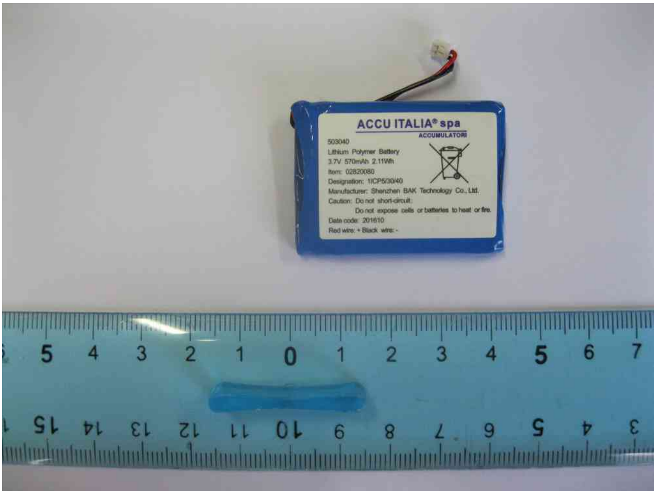
Fig. 13: Li-Pol Battery Top View
