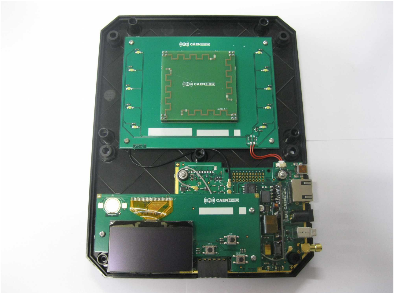
Figure 1: Internal view - Top Side
