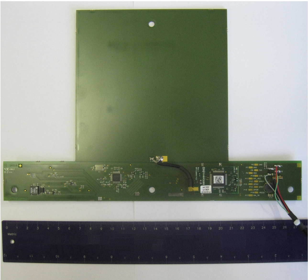
Figure 2: PCB bottom view
