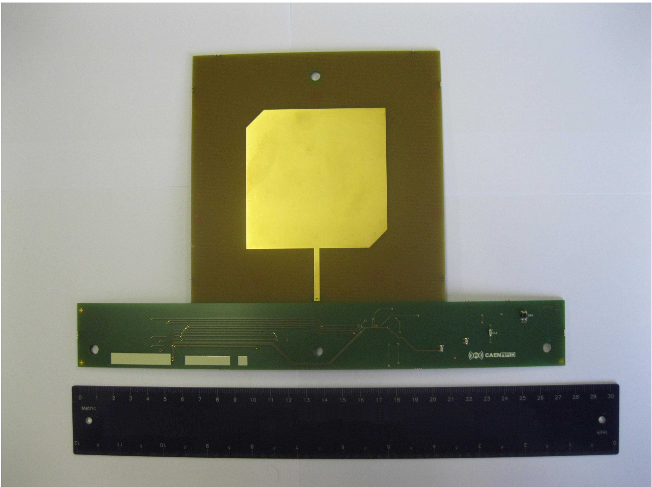
Figure 1: PCB top view
