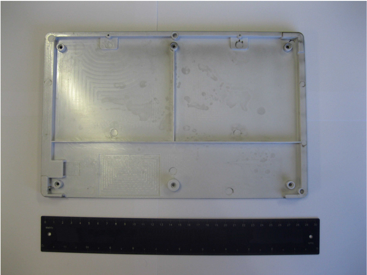
Figure 6: R1260UB –Bottom enclosure internal view
