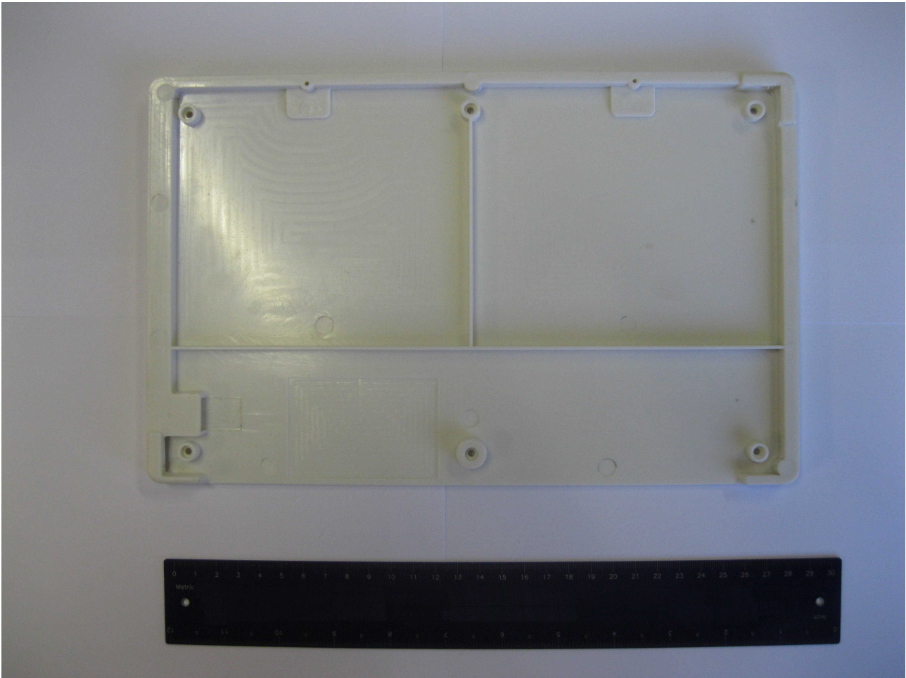
Figure 4: R1260U –Bottom enclosure internal view
