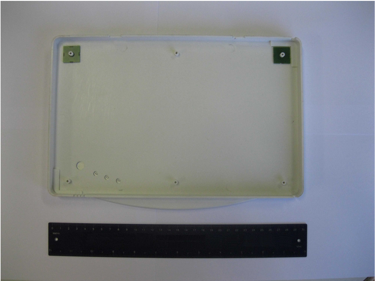
Figure 3: R1260U – Top enclosure internal view
