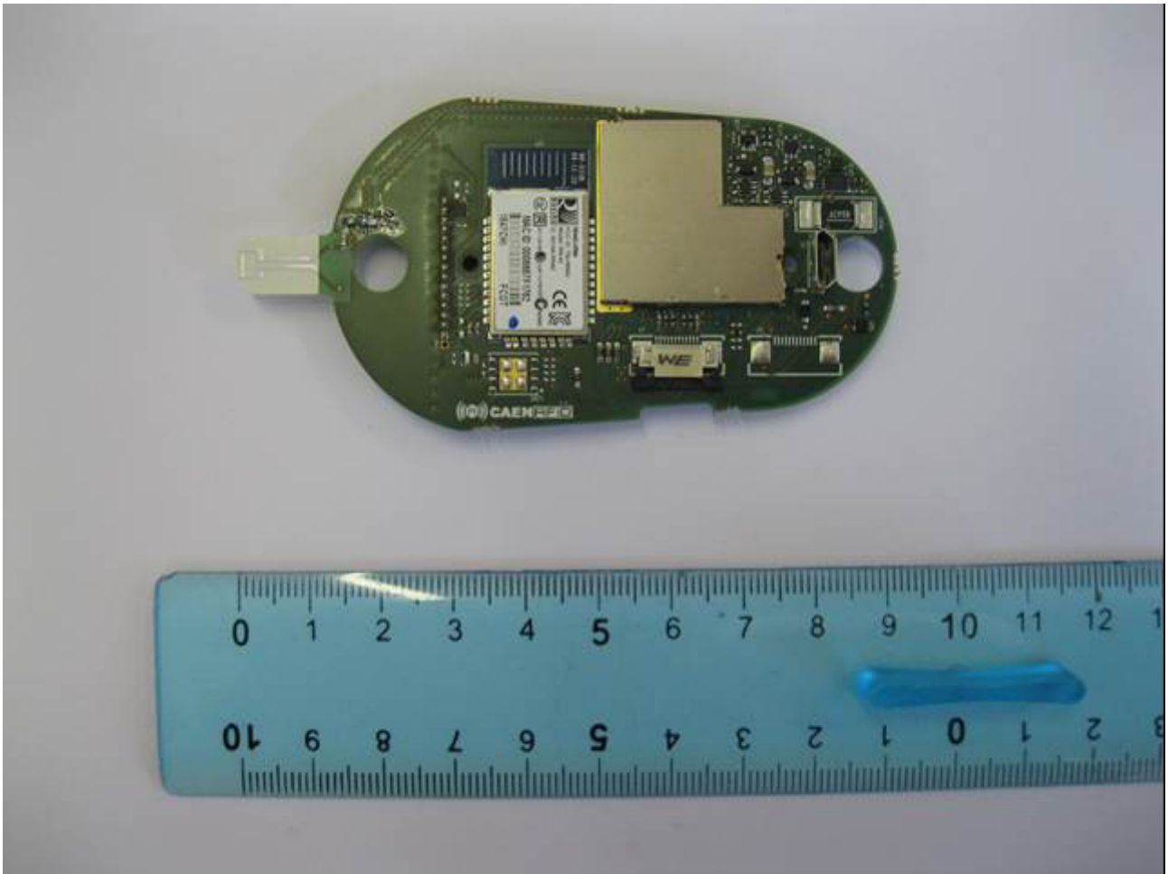
Fig. 4: PCB Bottom Side with shield installed
