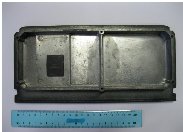
Fig. 7: Enclosure - BOTTOM side
