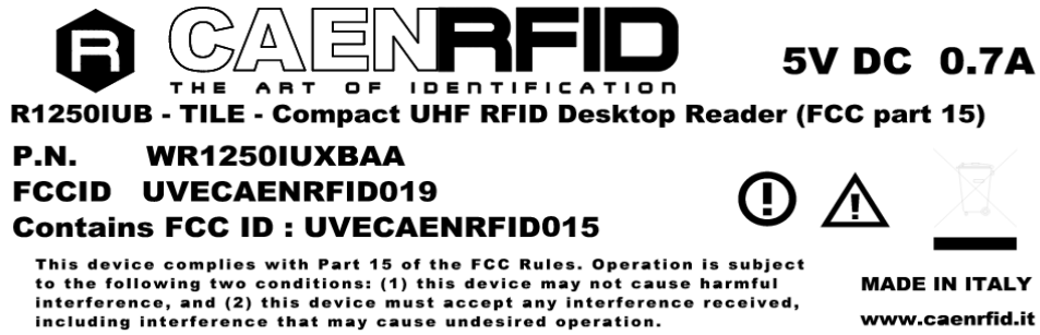
Fig. 3: Label of R1250IUB - Tile – Black - Compact UHF RFID Desktop Reader (FCC)
