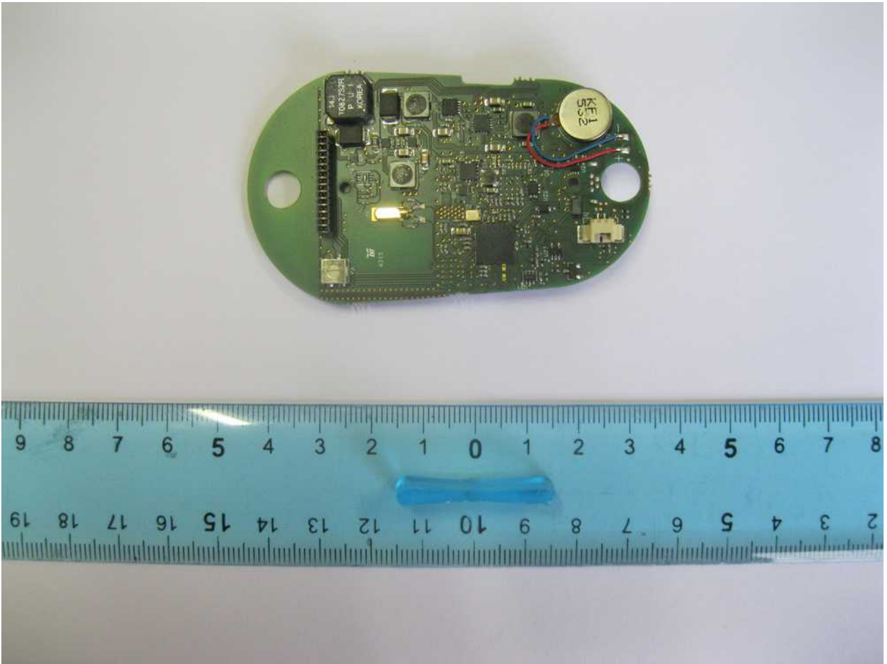
Fig. 2: R1170IUHIDP - PCB Top Side
