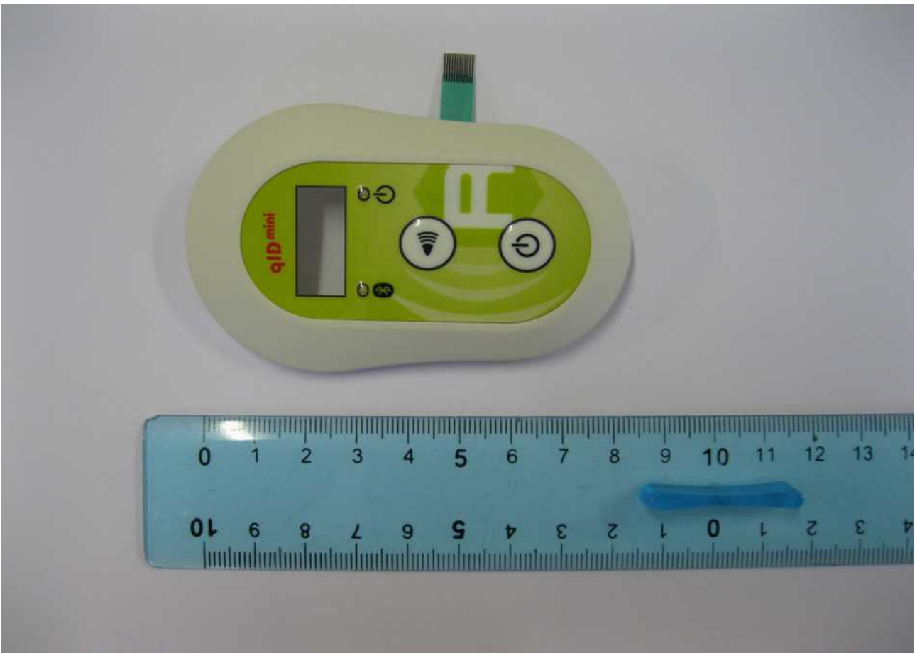
Fig. 7: Enclosure and keypad Top Side (external view)
