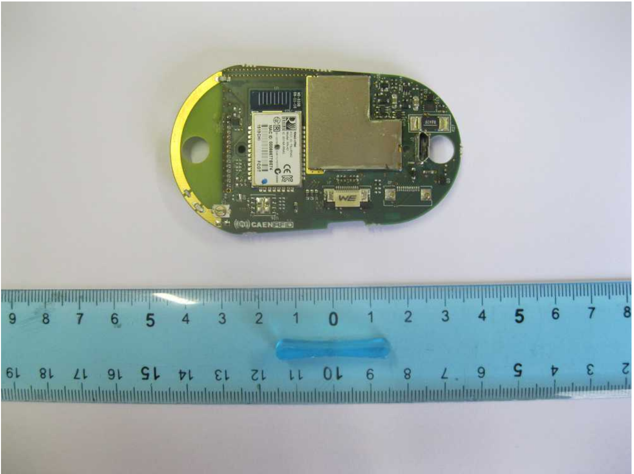
Fig. 5: R1170IUHIDP - PCB Bottom Side
