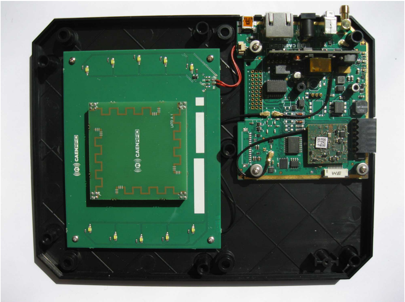
Figure 3 - Host board with RF switch
