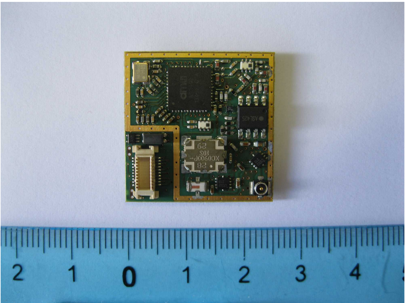
Figure 1 - R1270C Module Top View
