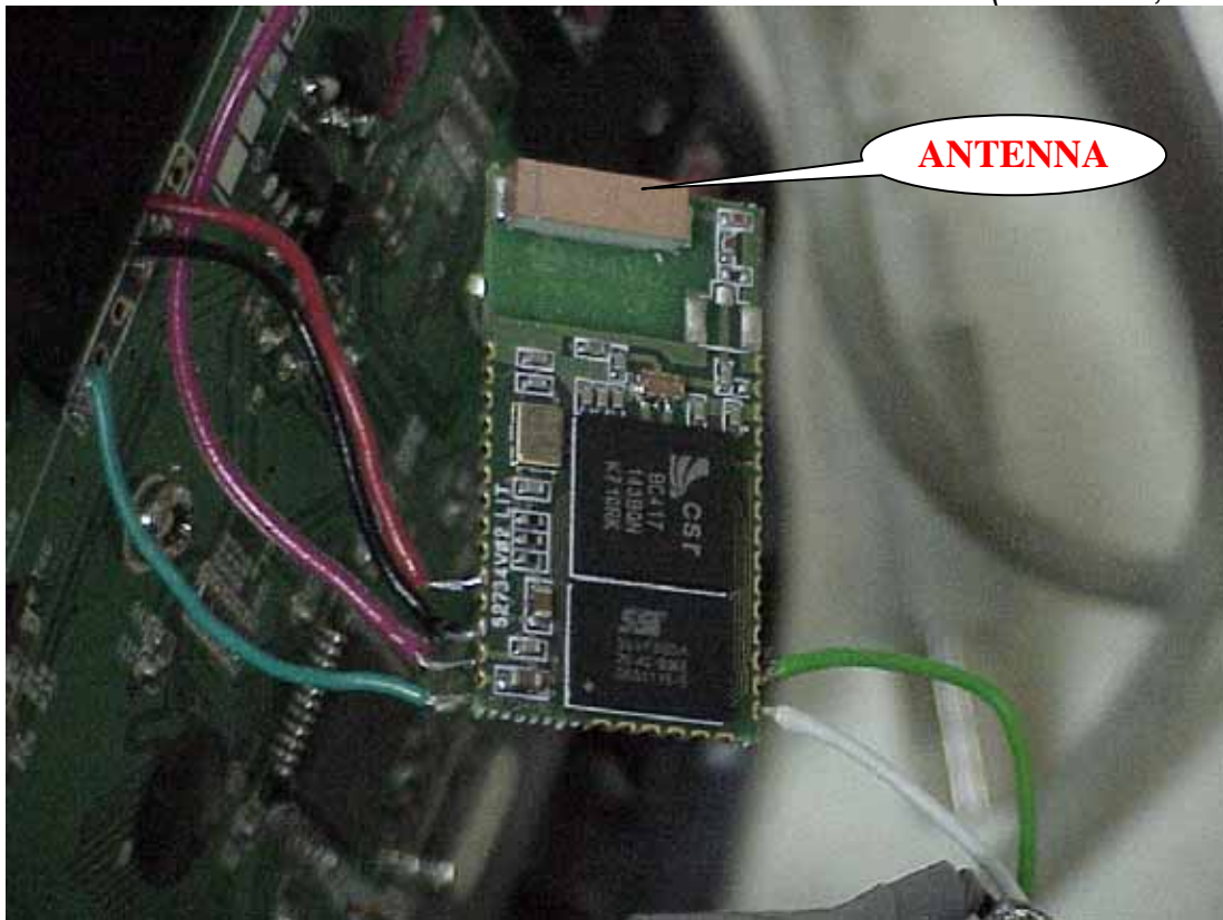
Figure 10 Internal View (RF Board, Front View)
