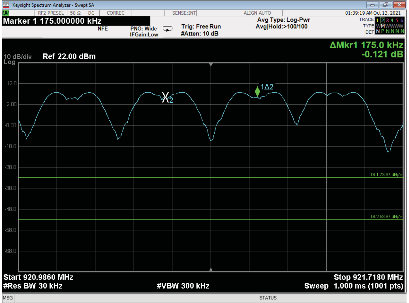
Channel Frequency Separation – Hop Set 3
