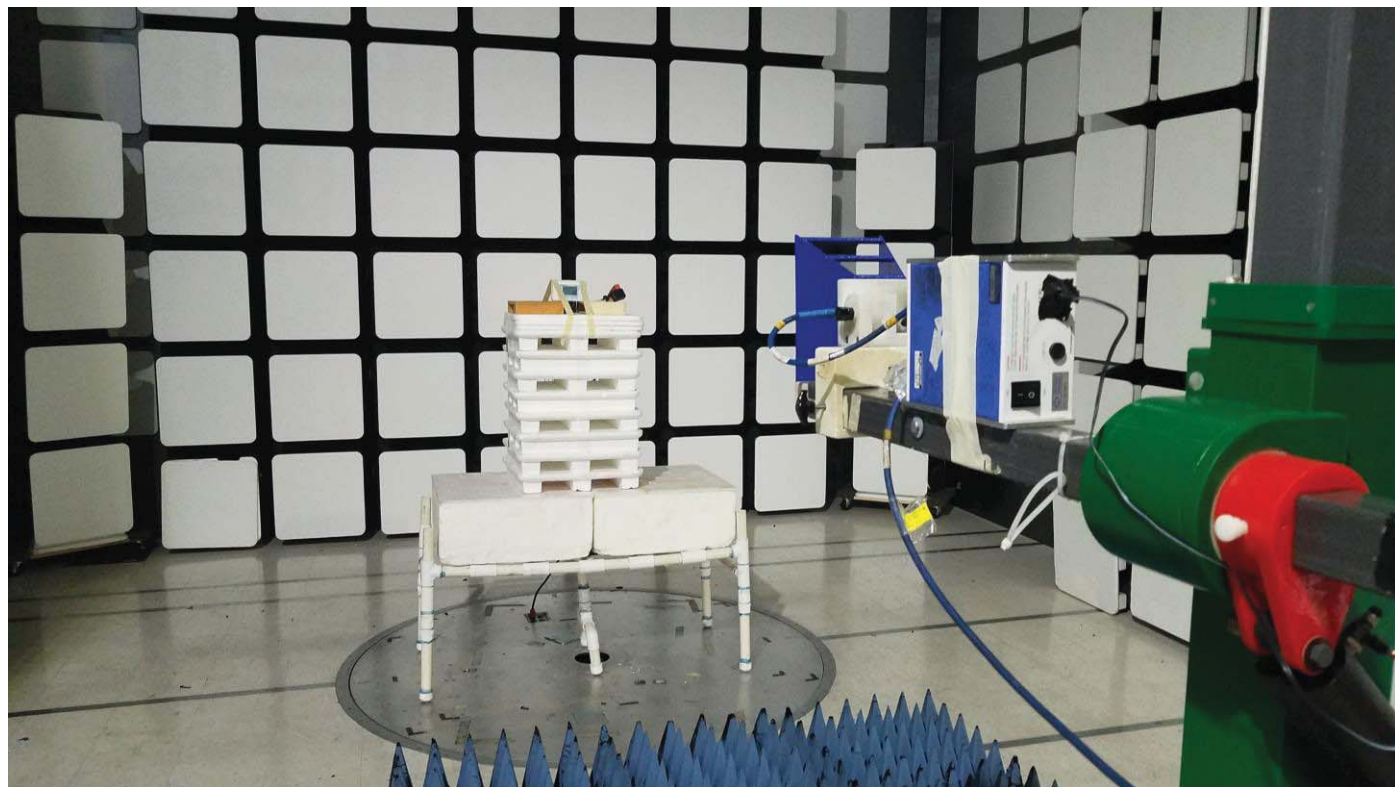
FRONT VIEW
