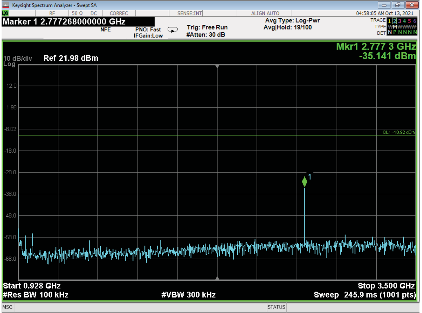
RF Antenna Conducted – High Channel – 928 MHz to 3.5 GHz
