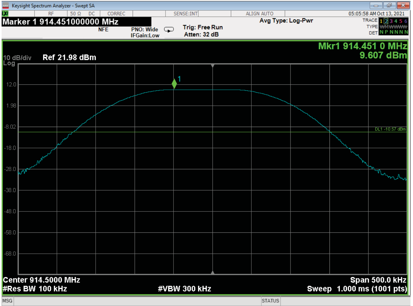
RF Antenna Conducted – Middle Channel – Reference Level
