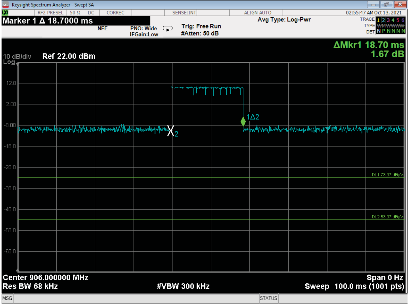
Time of One Pulse – 18.7 ms
