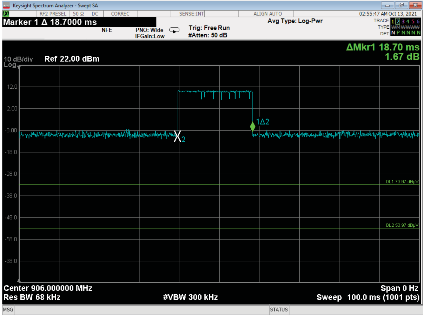
Time of One Pulse – 18.7 ms
