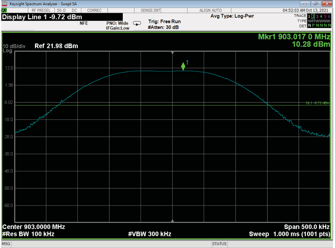
RF Antenna Conducted – Low Channel Reference Level
