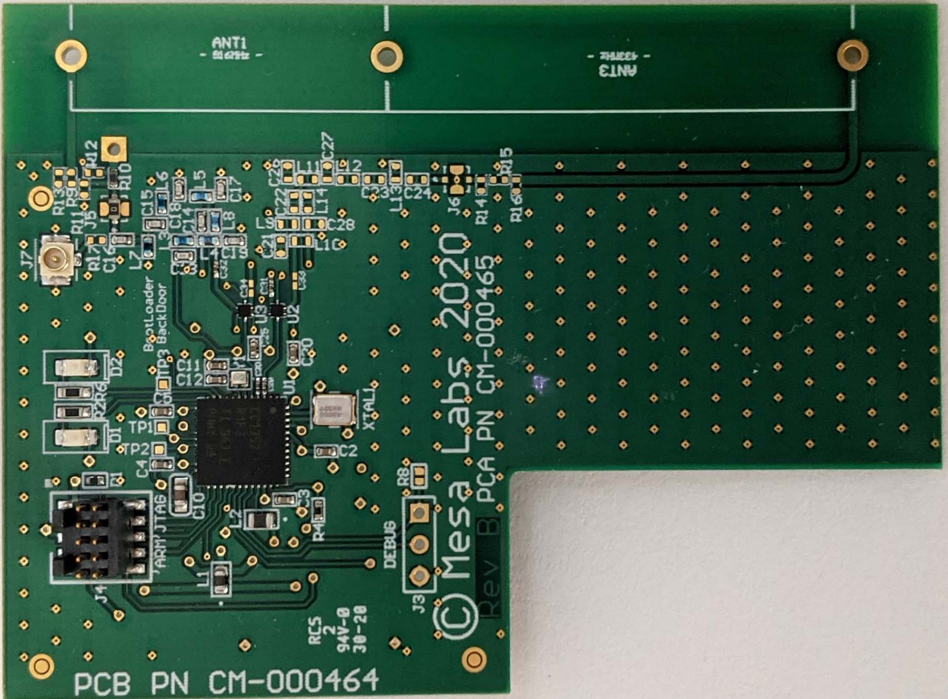
Top View of the RF Module
