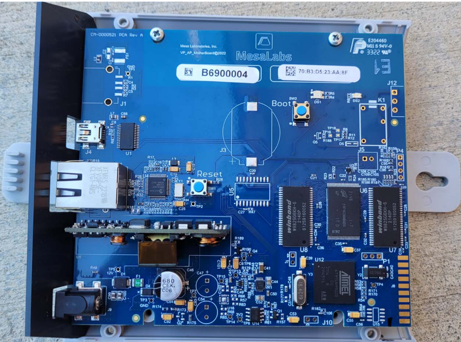
Inside View of the EUT
