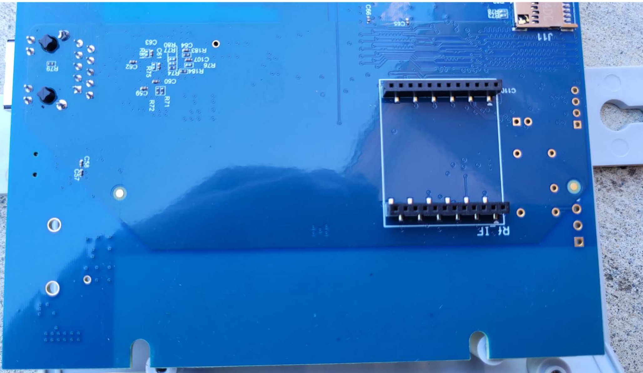
Bottom View of the PCB - Closeup #4
