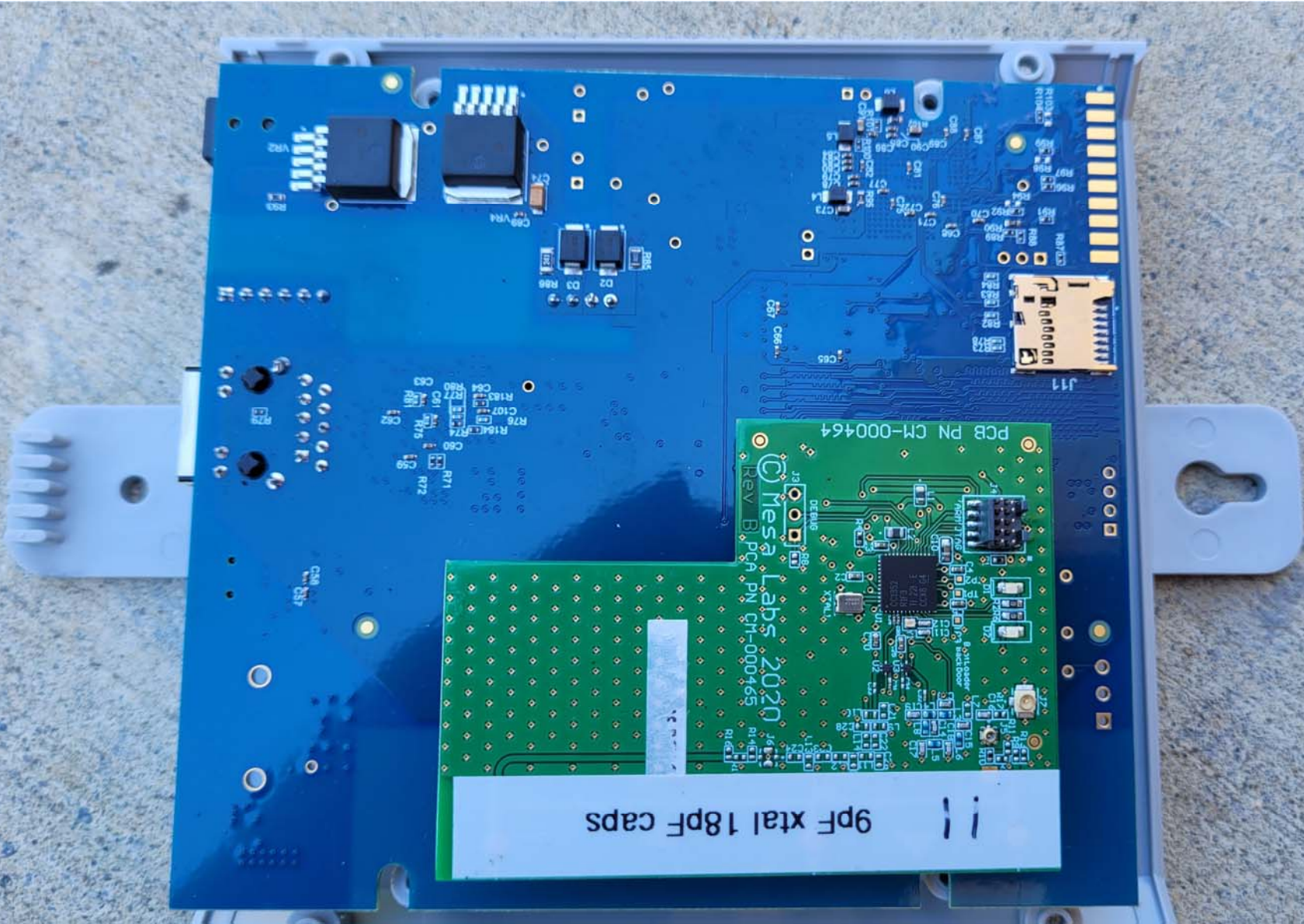
Bottom View of the PCB with RF Board
