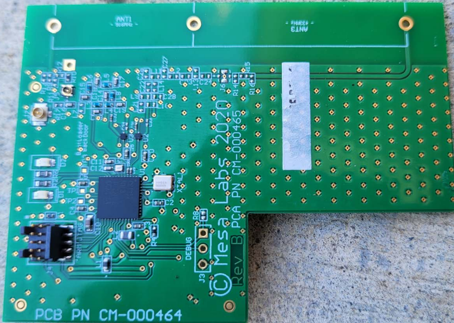
Top View of the RF Board
