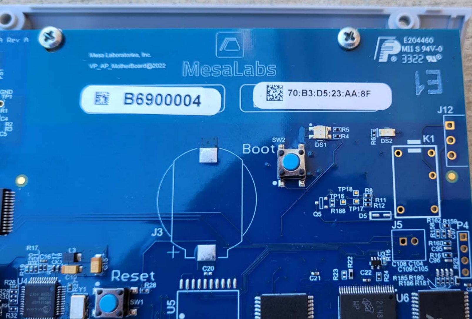
Top View of the PCB - Closeup #6
