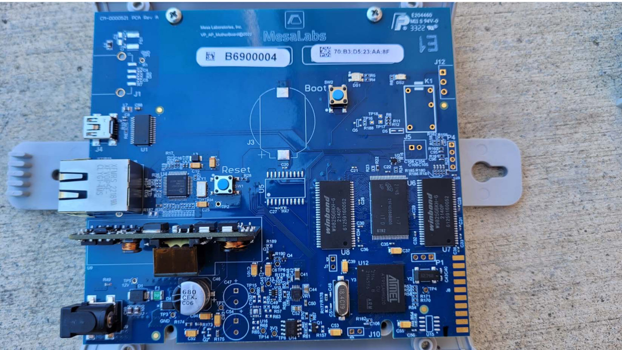
Top View of the PCB for the EUT
