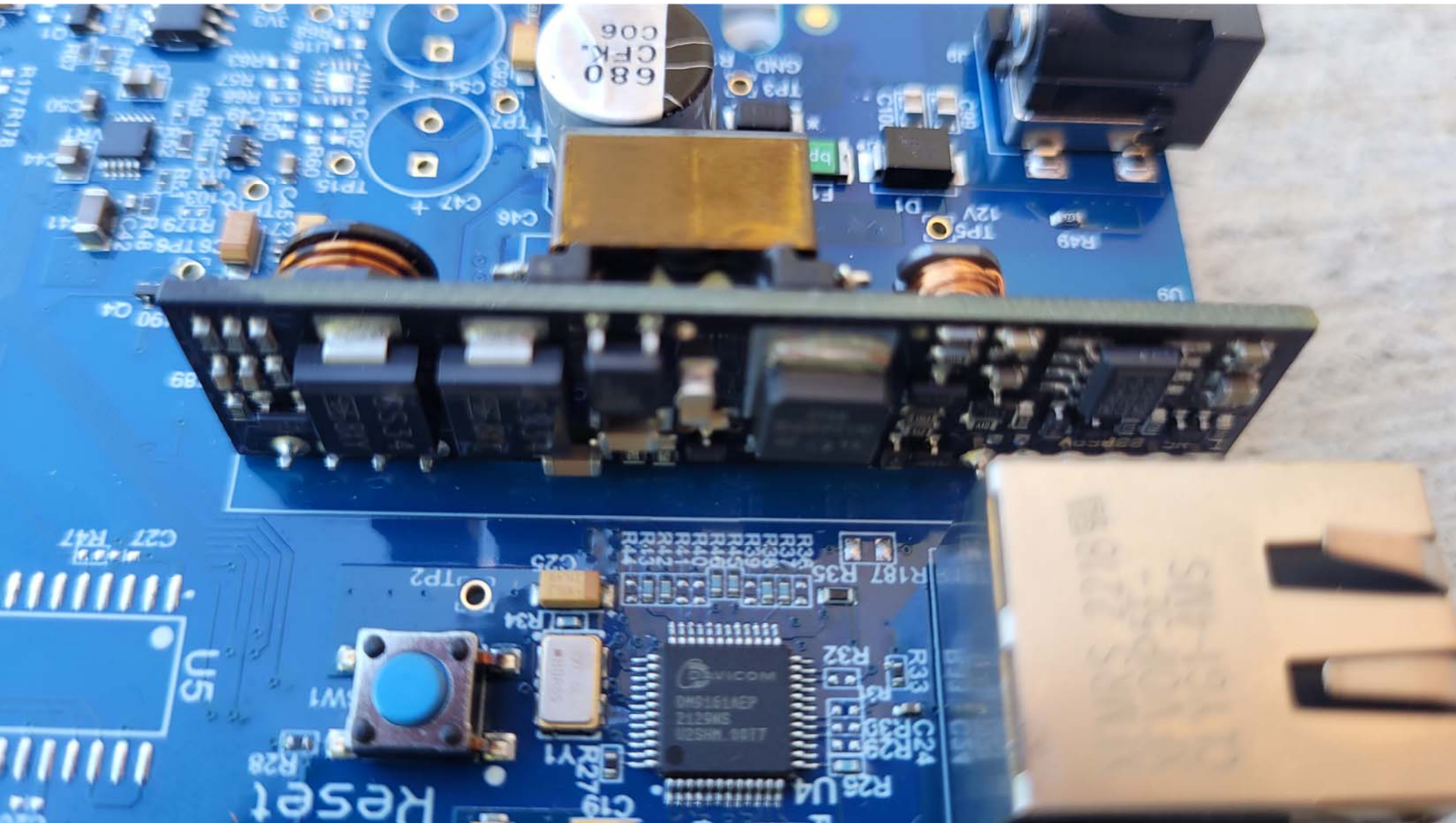
View of the Large Board - Top Side
