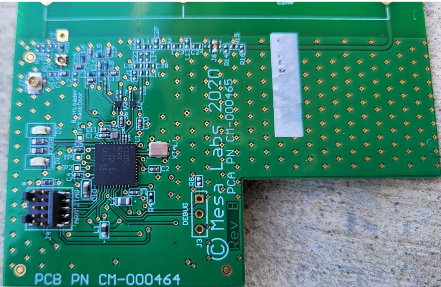
Top View of the RF Board - View #2
