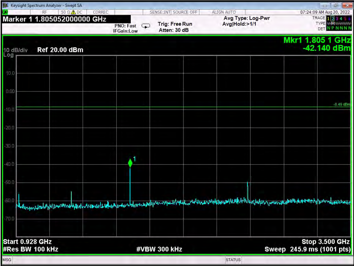
RF Antenna Conducted - Low Channel - G4 Compatibility Mode - 928 MHz to 3.5 GHz
