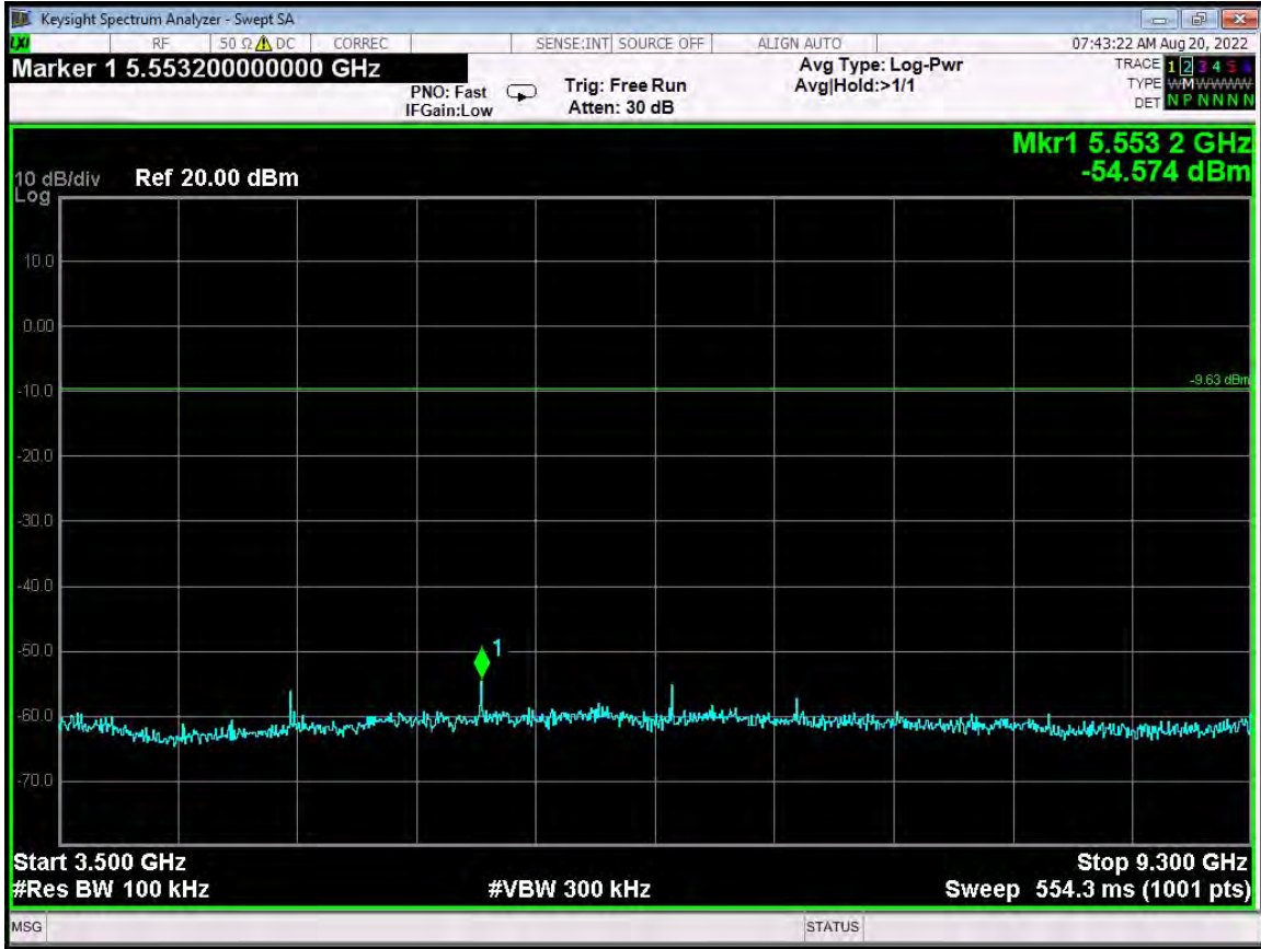
RF Antenna Conducted - High Channel - G4 Compatibility Mode - 3.5 GHz to 9.3 GHz
