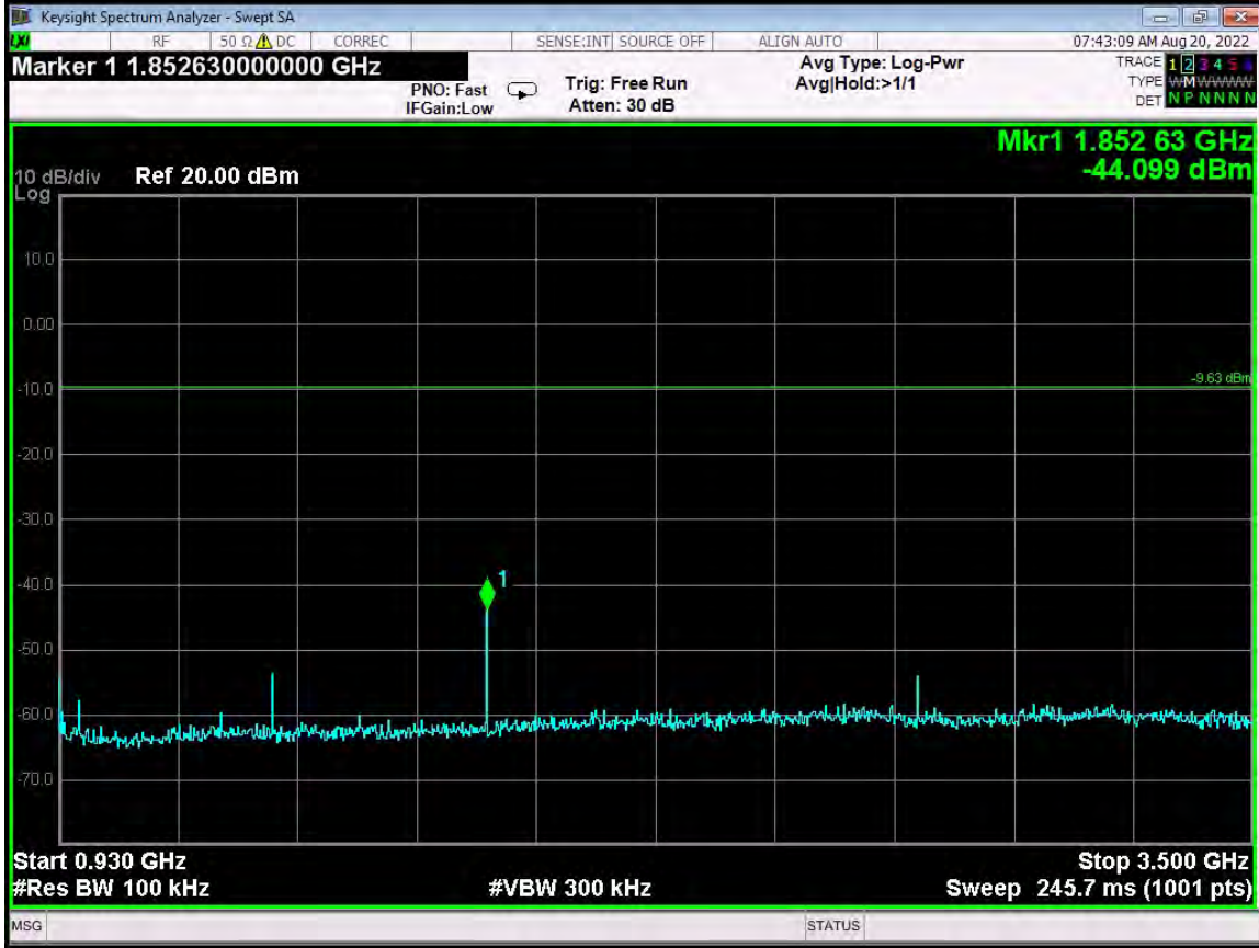
RF Antenna Conducted - High Channel - G4 Compatibility Mode - 930 MHz to 3.5 GHz
