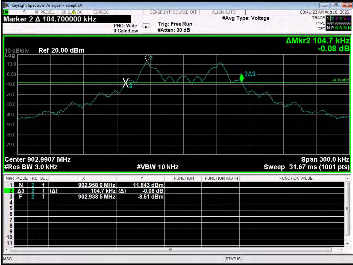
-20 dB Bandwidth - 903.00 MHz - G4 Compatibility Mode - 104.7 kHz
