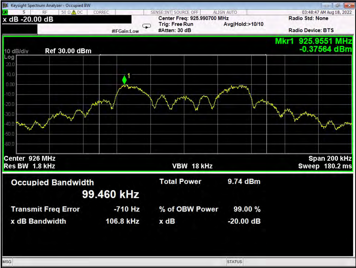
99 % Bandwidth - 926.00 MHz - G4 Compatibility Mode
