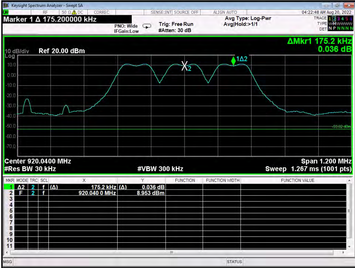
Channel Frequency Separation - Hop Set 3 - G4 Compatibility Mode
