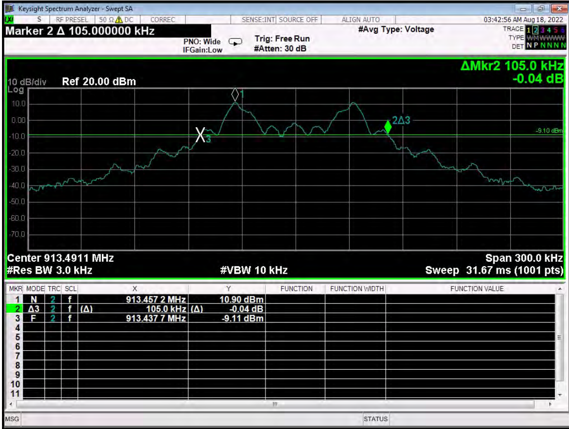
-20 dB Bandwidth - 913.50 MHz - G4 Compatibility Mode - 105.0 kHz
