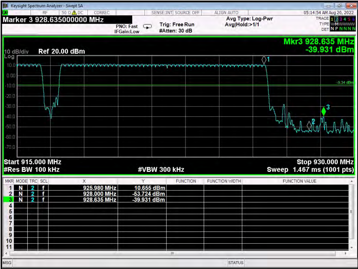
Band Edge – High Channel - G4 Compatibility Mode - Frequency Hopping - Hop Set 3 Worst Case
