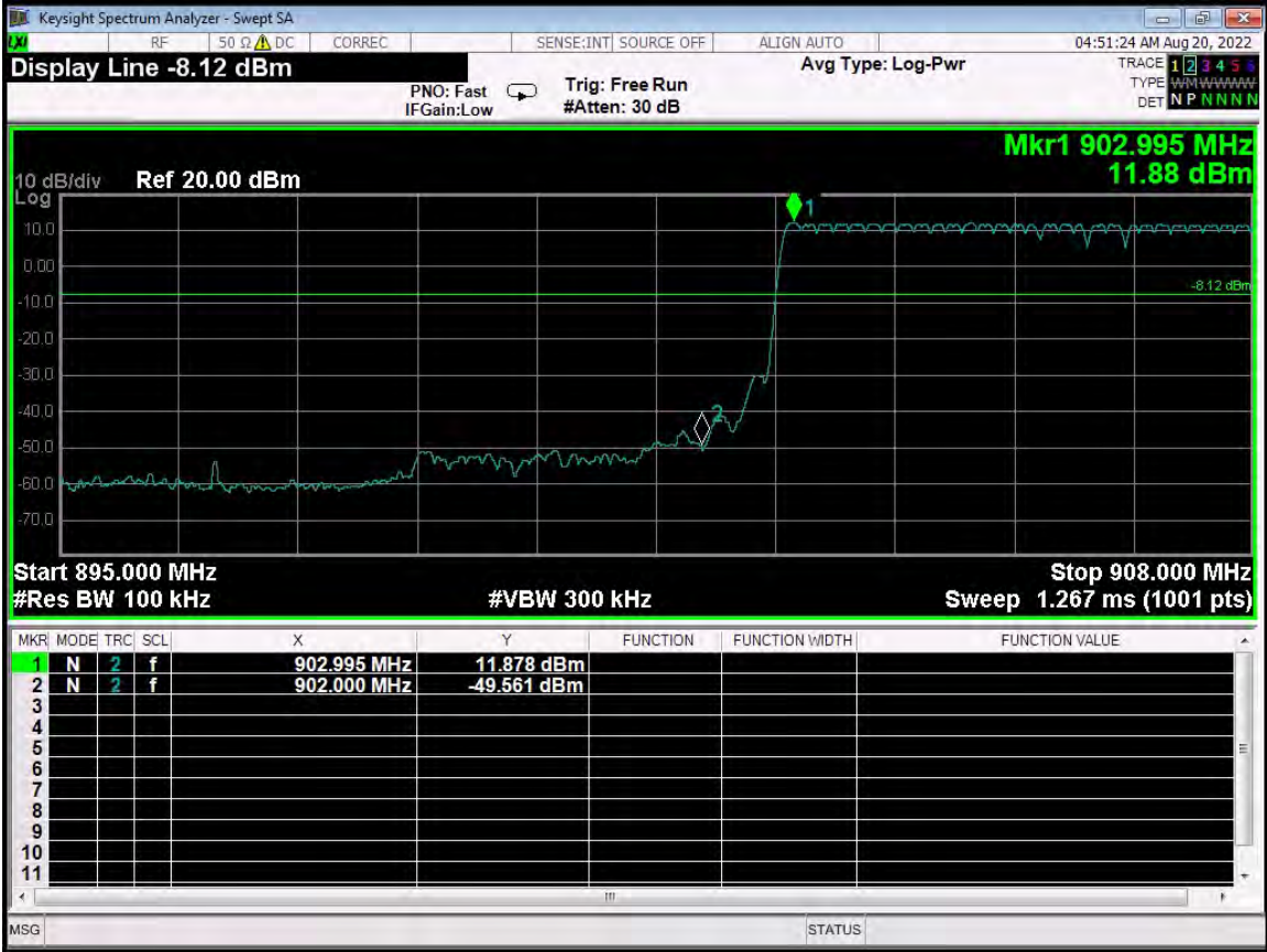
Band Edge – Low Channel - G4 Compatibility Mode - Frequency Hopping - Hop Set 2 Worst Case
