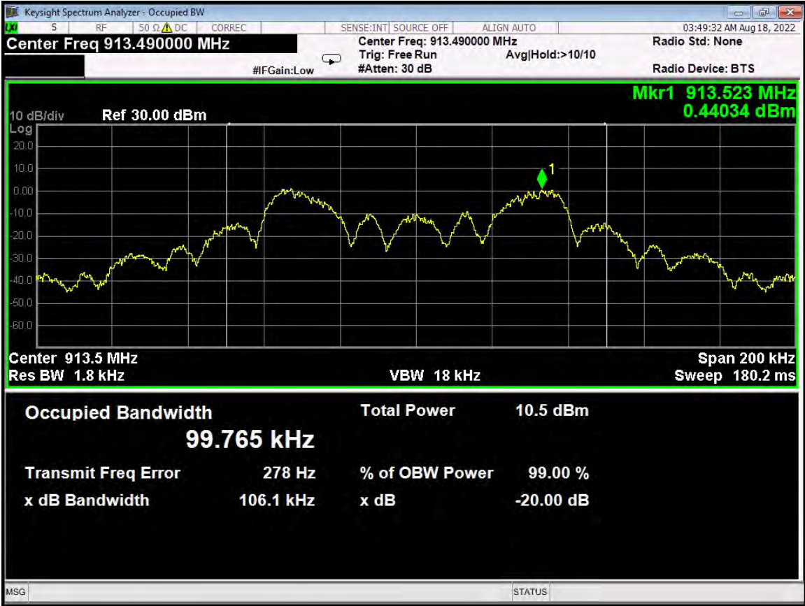
99 % Bandwidth - 913.50 MHz - G4 Compatibility Mode
