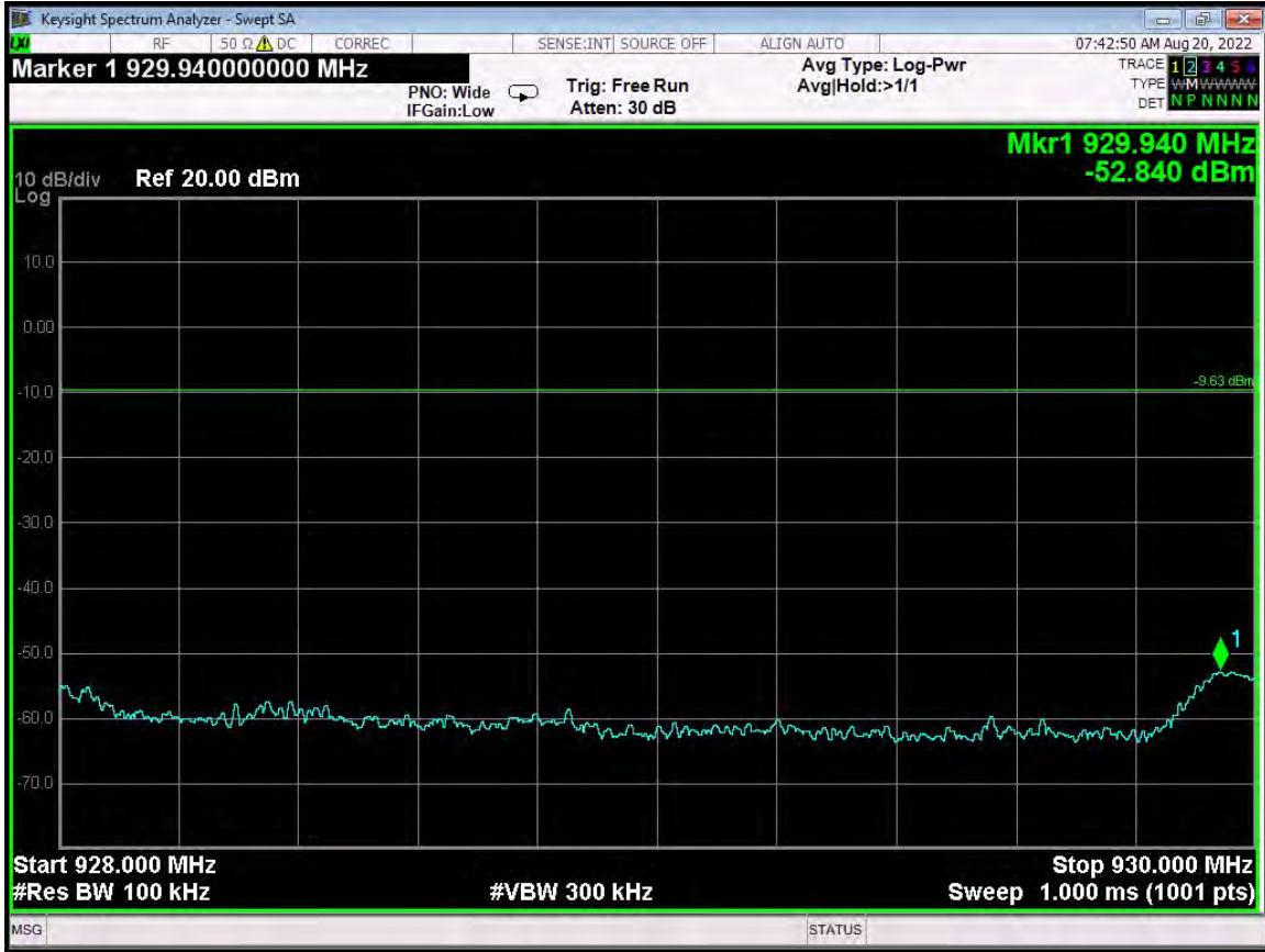
RF Antenna Conducted - High Channel - G4 Compatibility Mode - 928 MHz to 930 MHz
