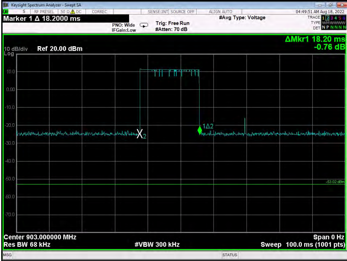
Time of One Pulse - 18.2 ms - Worst Case Mode of Hop Set 1 - G4 Compatibility Mode
