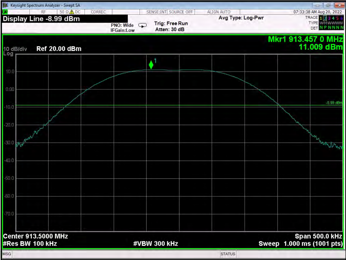
RF Antenna Conducted - Mid Channel - G4 Compatibility Mode - Reference Level
