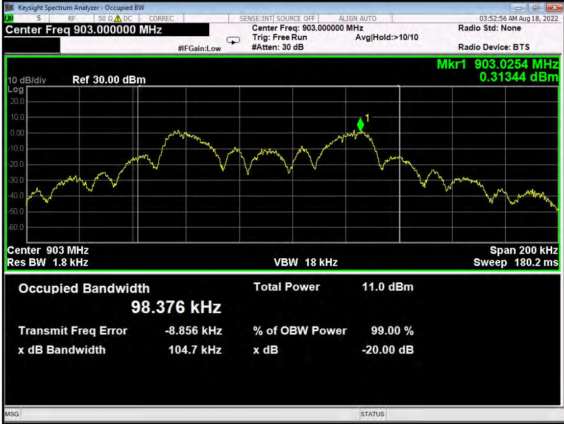
99 % Bandwidth - 903.00 MHz - G4 Compatibility Mode
