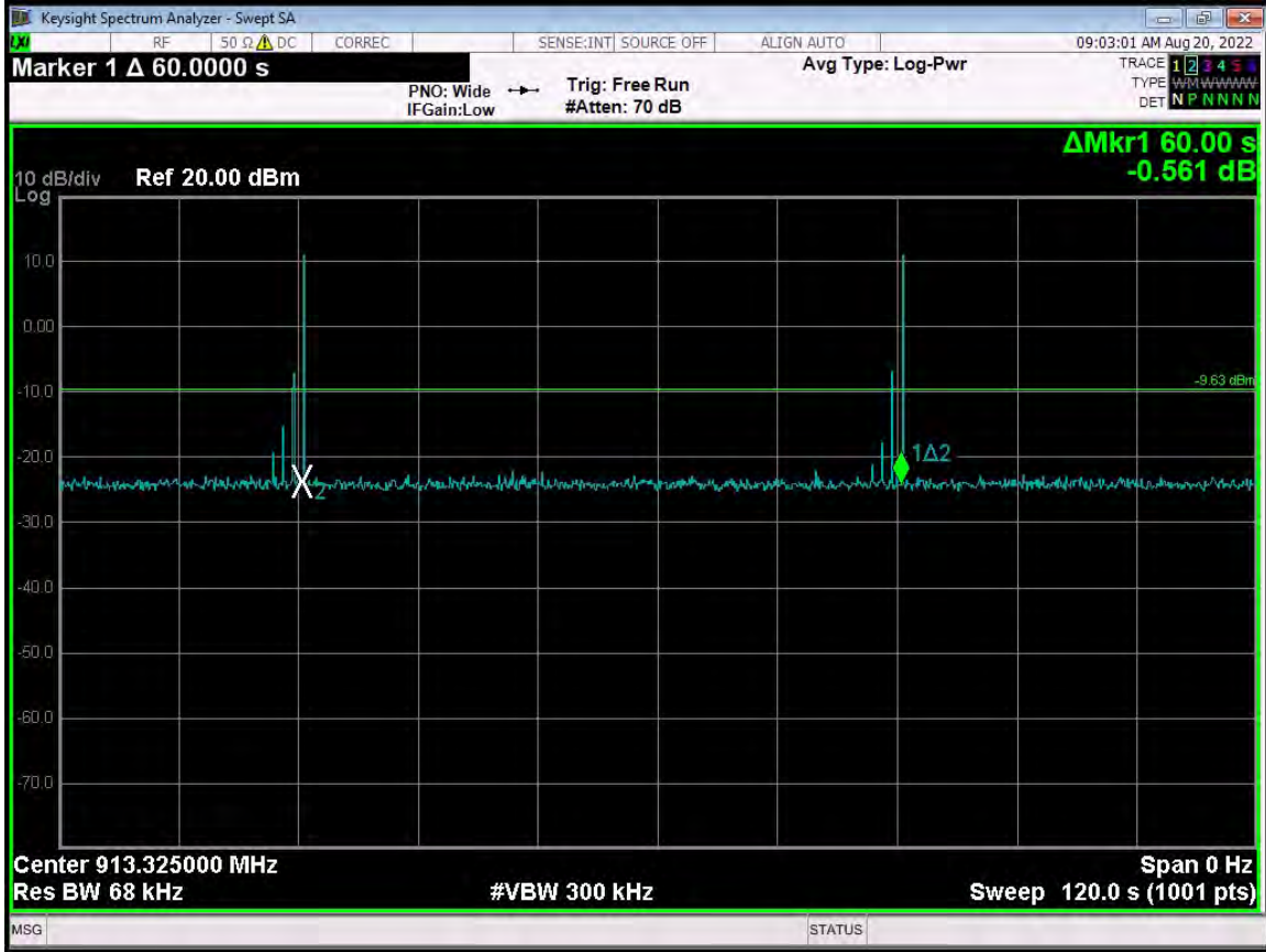
Time Between Pulses - 60 Seconds - Hop Set 2 - G4 Compatibility Mode
