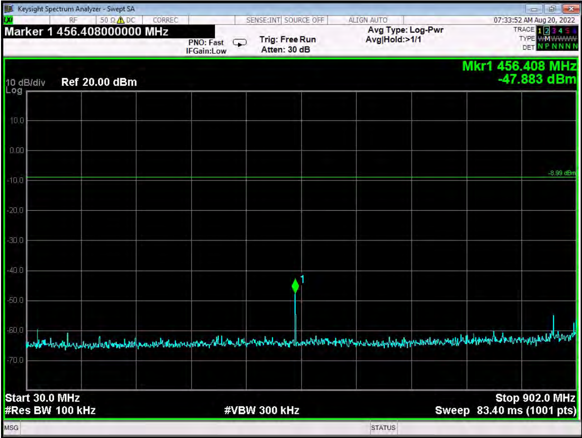
RF Antenna Conducted - Mid Channel - G4 Compatibility Mode - 30 MHz to 902 MHz
