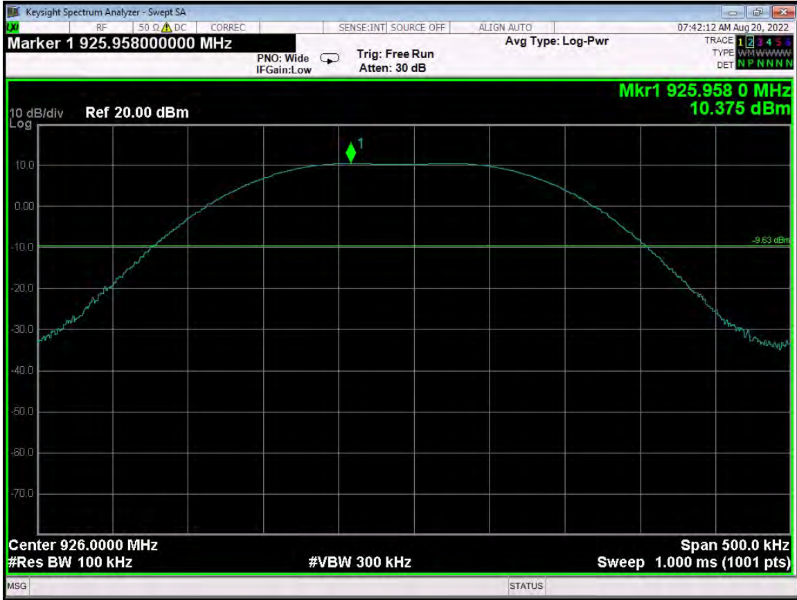
RF Antenna Conducted - High Channel - G4 Compatibility Mode - Reference Level
