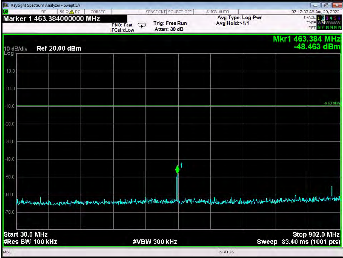
RF Antenna Conducted - High Channel - G4 Compatibility Mode - 30 MHz to 902 MHz
