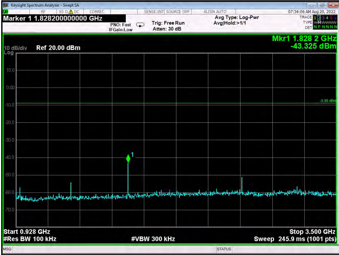
RF Antenna Conducted - Mid Channel - G4 Compatibility Mode - 928 MHz to 3.5 GHz
