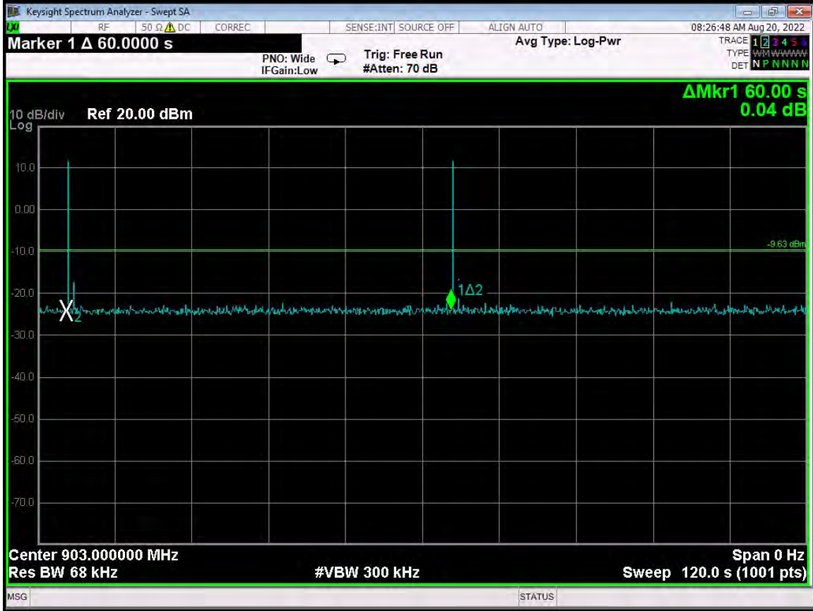
Time Between Pulses - 60 Seconds - Hop Set 1 - G4 Compatibility Mode
