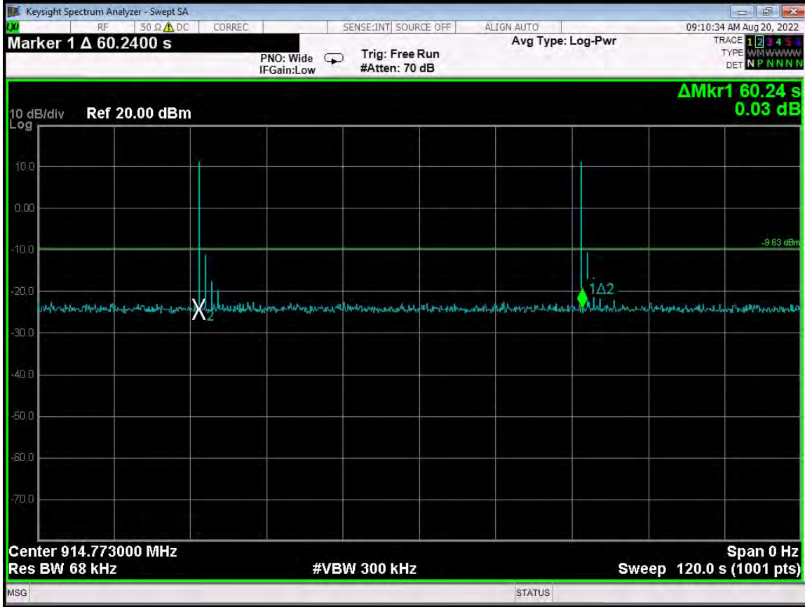
Time Between Pulses – 60.24 Seconds - Hop Set 3 - G4 Compatibility Mode
