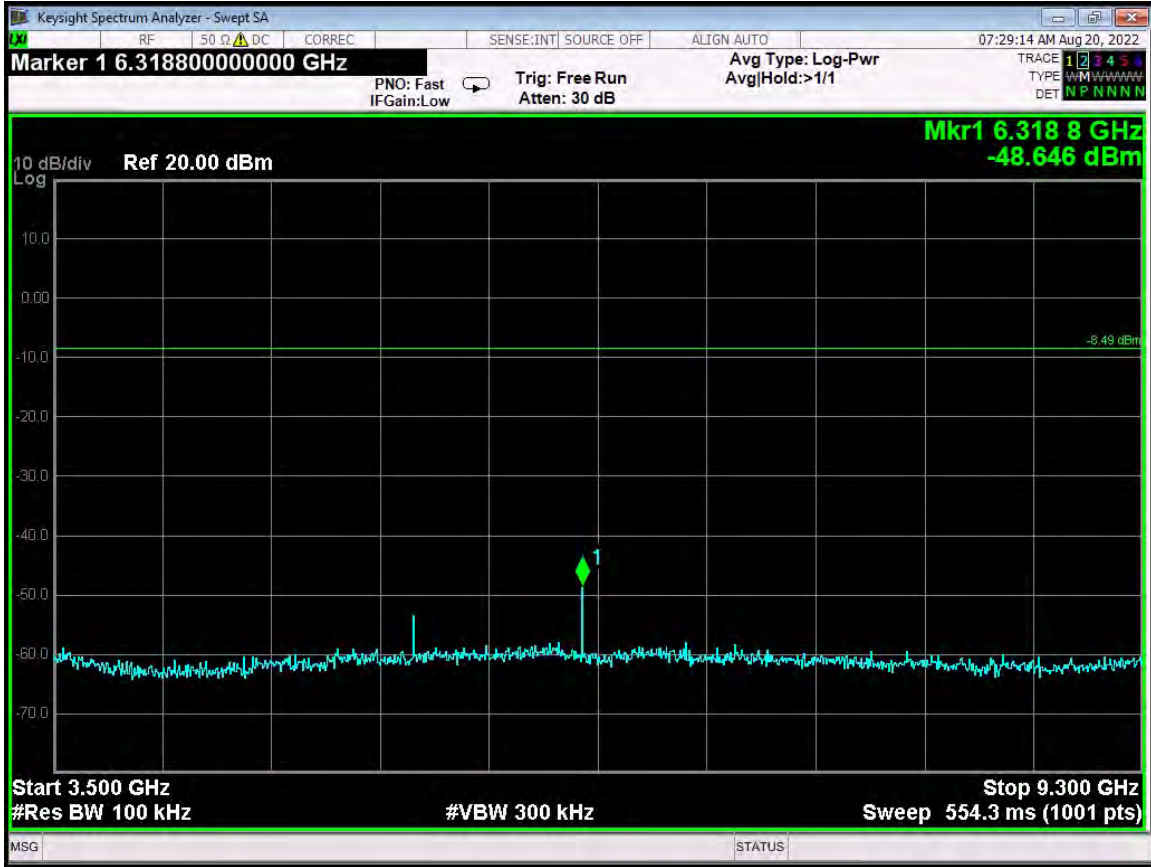
RF Antenna Conducted - Low Channel - G4 Compatibility Mode - 3.5 GHz to 9.3 GHz
