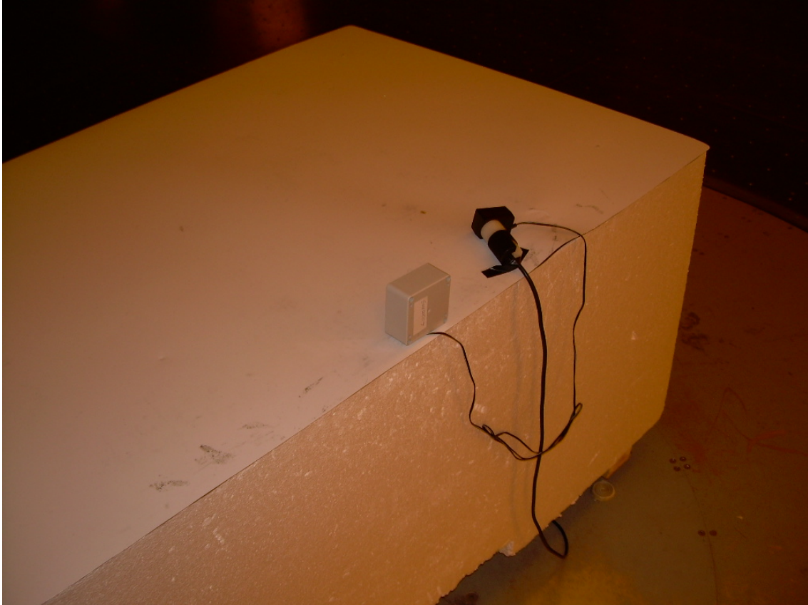
Photograph 4 - Back View Radiated Spurious Worst-Case Configuration - DTENV-R
