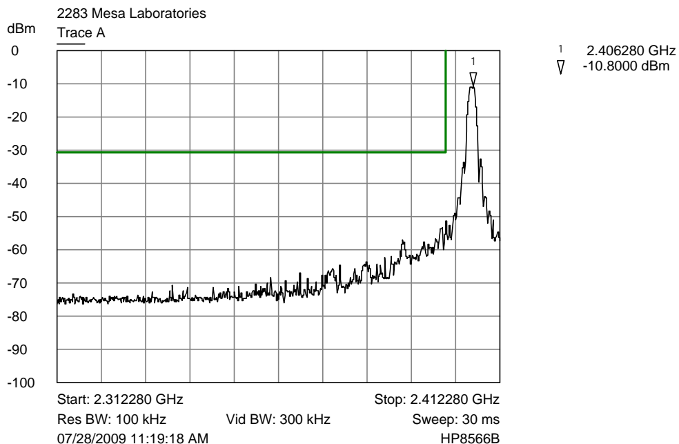
Trace A Lower channel band edge plot (1/1 power setting)
