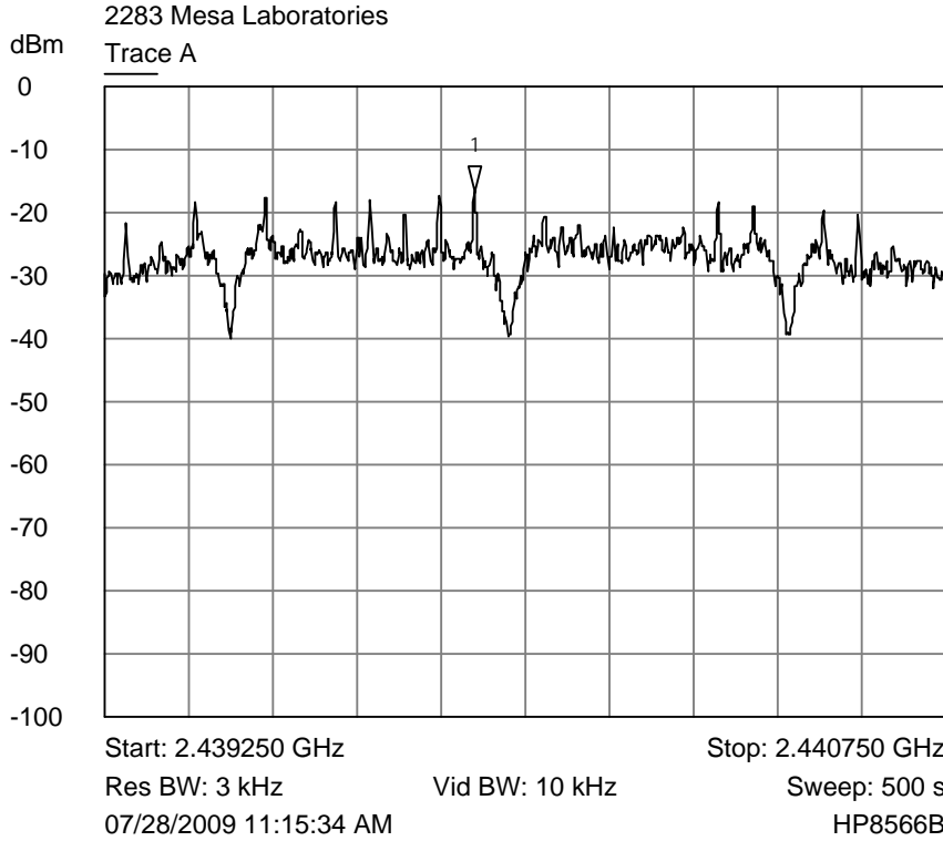
Trace A Middle channel 3 kHz power spectral density plot (1/1 power setting)
