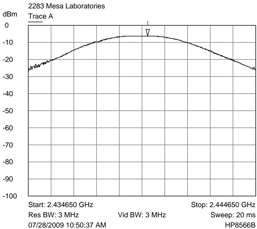
Trace A Middle channel output power plot (1/1 power setting)
