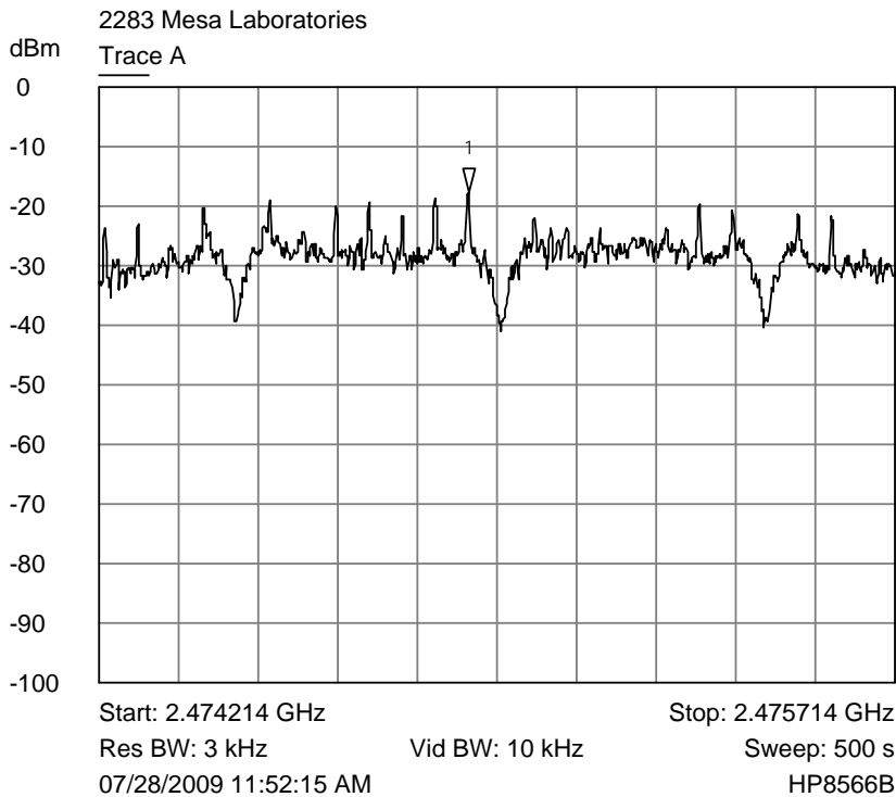
Trace A Upper channel 3 kHz power spectral density plot (1/1 power setting)
