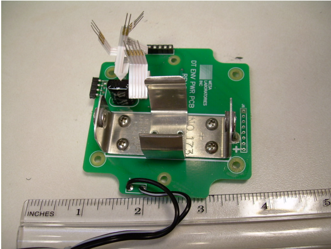
Photograph 20 - Top Side of the Main PCB of the DTENV-R
