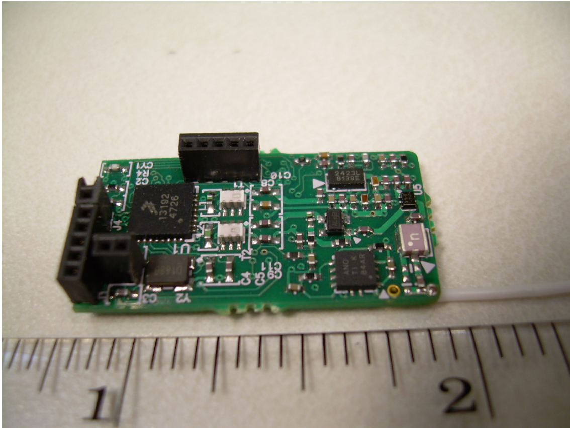
Photograph 15 - Top Side of the Transceiver PCB
