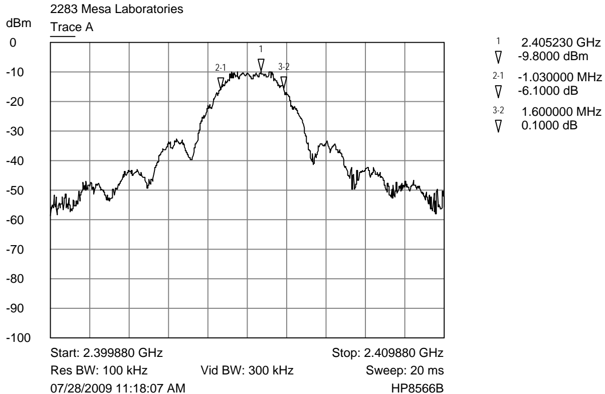
Trace A Lower channel bandwidth plot (1/1 power setting)
