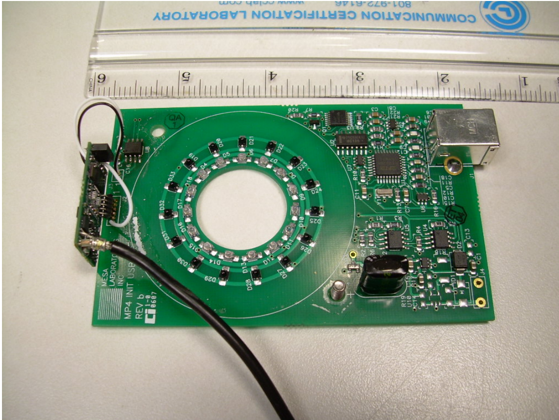
Photograph 12 - Component Side of the Main PCB of the DTENV-H with Reflector Removed
