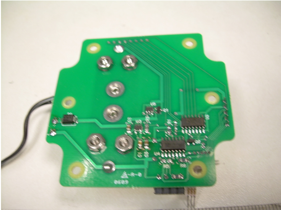
Photograph 21 - Bottom Side of the Main PCB of the DTENV-R
