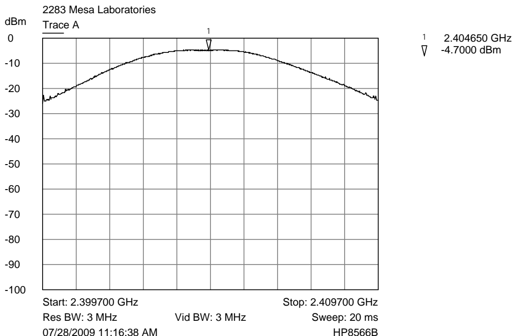
Trace A Lower channel output power plot (1/1 power setting)
