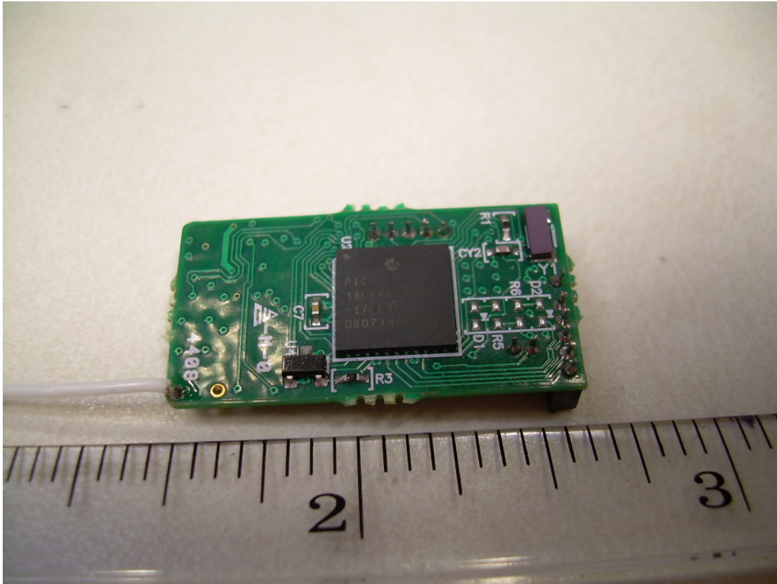
Photograph 16 - Bottom Side of the Transceiver PCB
