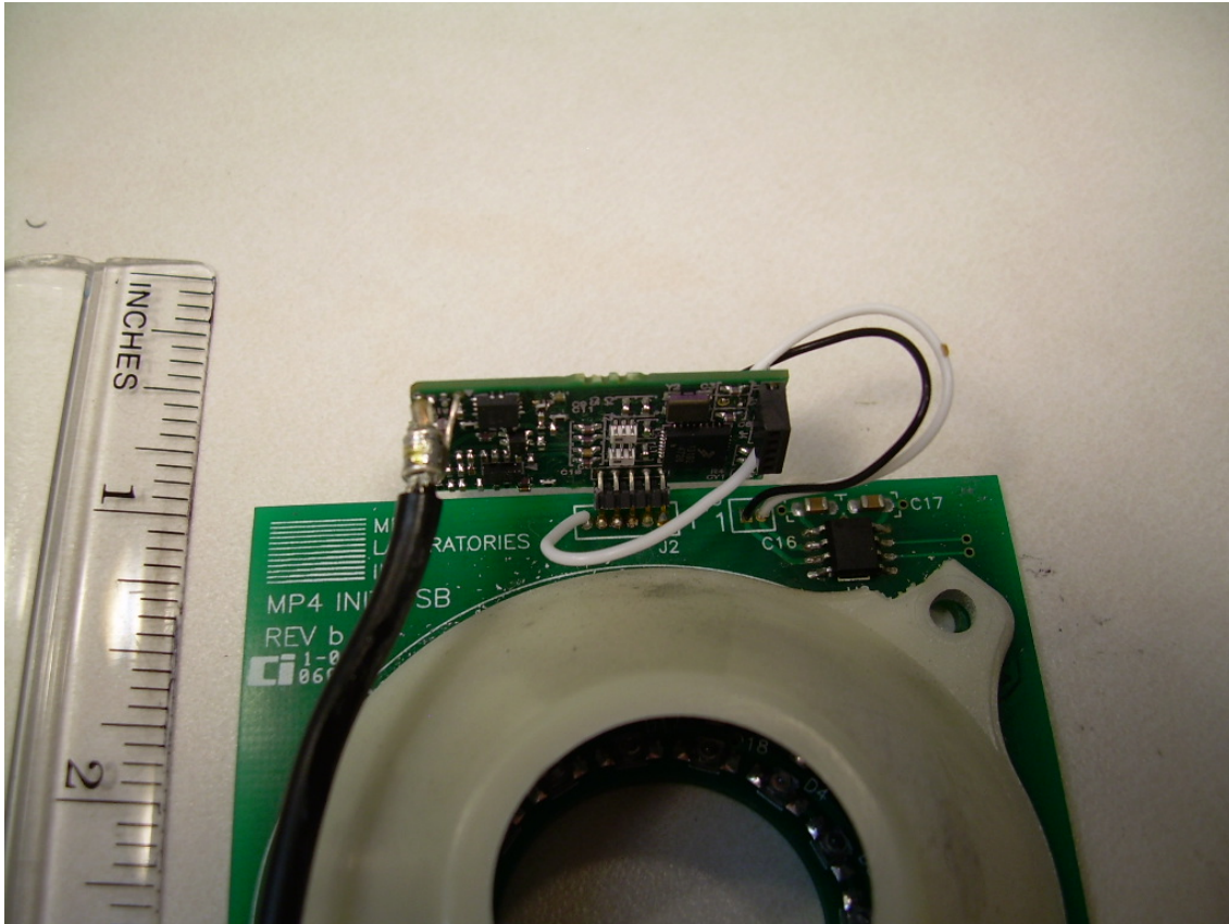
Photograph 14 - Placement of the Transceiver PCB in the DTENV-H
