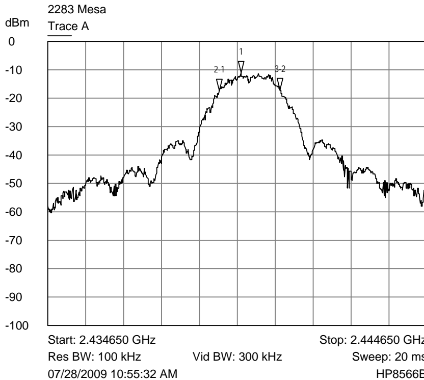
Trace A Middle channel bandwidth plot (1/1 power setting)
