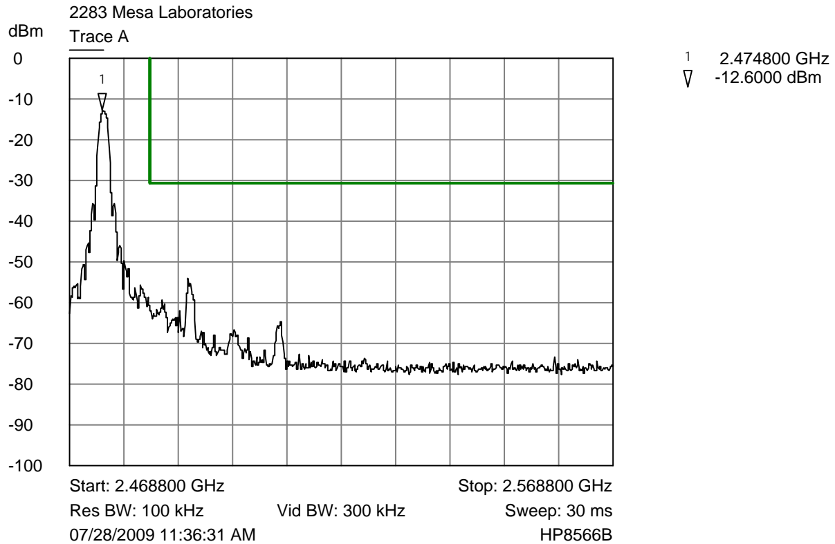
Trace A Upper channel band edge plot (1/1 power setting)
