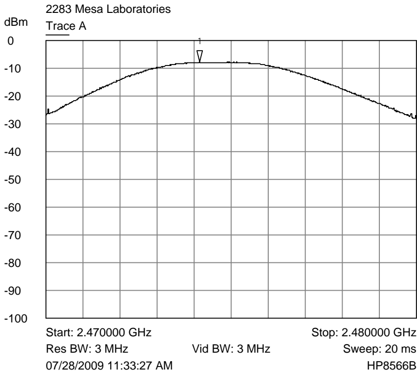
Trace A Upper channel output power plot (1/1 power setting)
