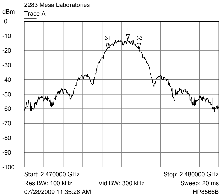
Trace A Upper channel bandwidth plot (1/1 power setting)
