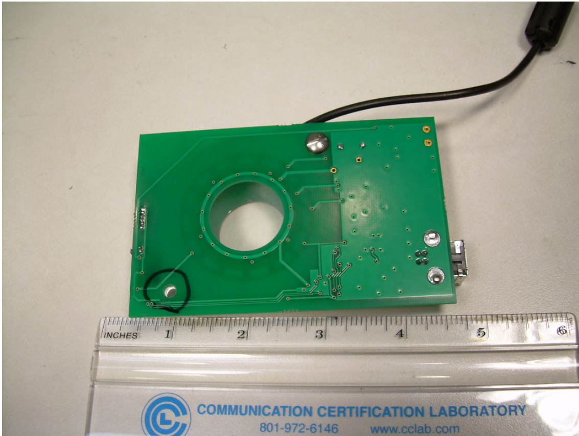
Trace Side of the Main PCB of the DTENV-H
