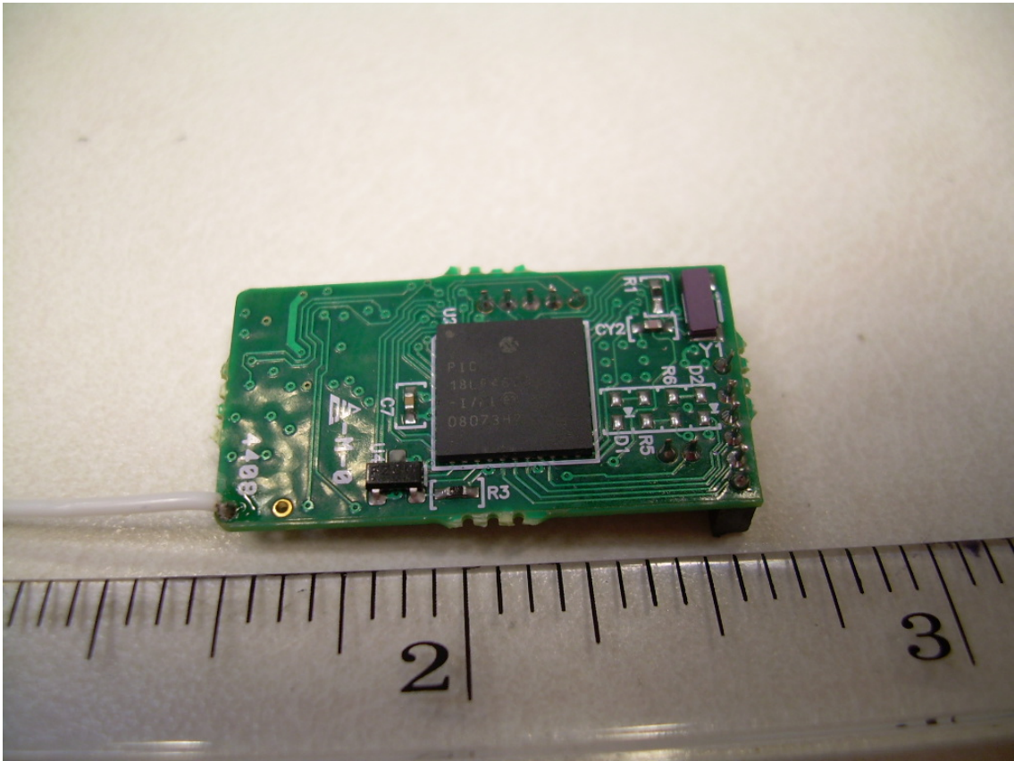
Bottom Side of the Transceiver PCB
