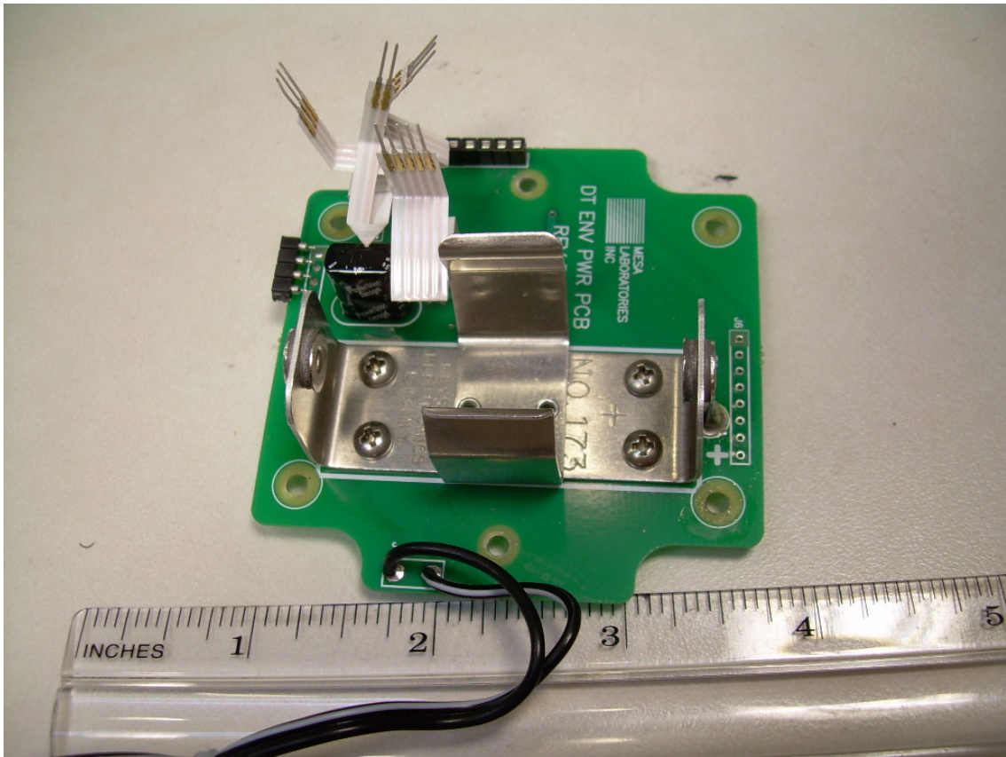
Top Side of the Main PCB of the DTENV-R
