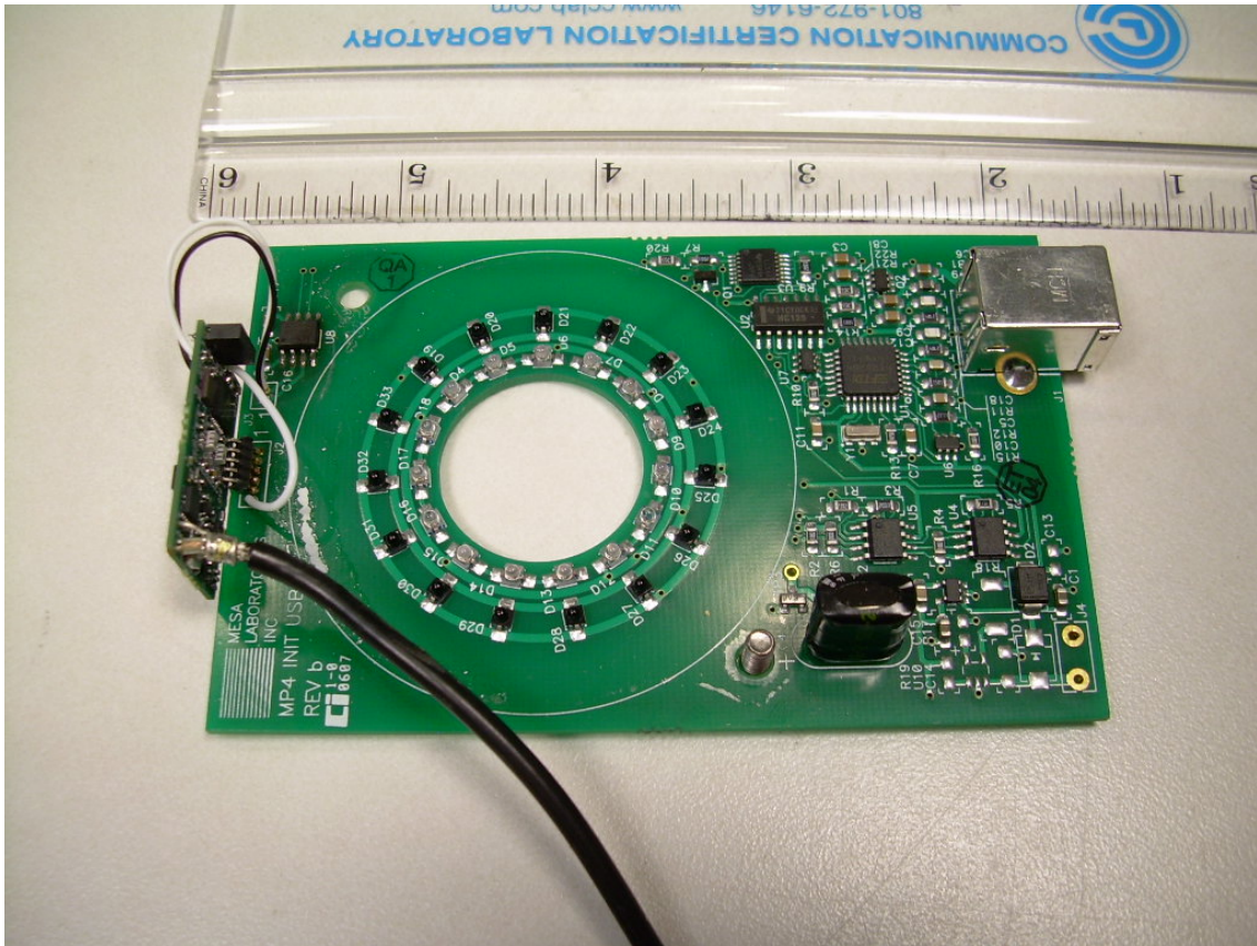
Component Side of the Main PCB of the DTENV-H with Reflector Removed
