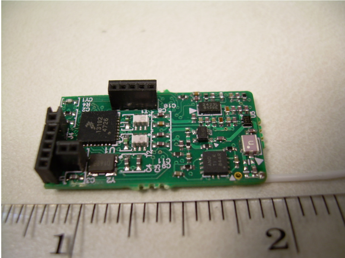
Top Side of the Transceiver PCB
