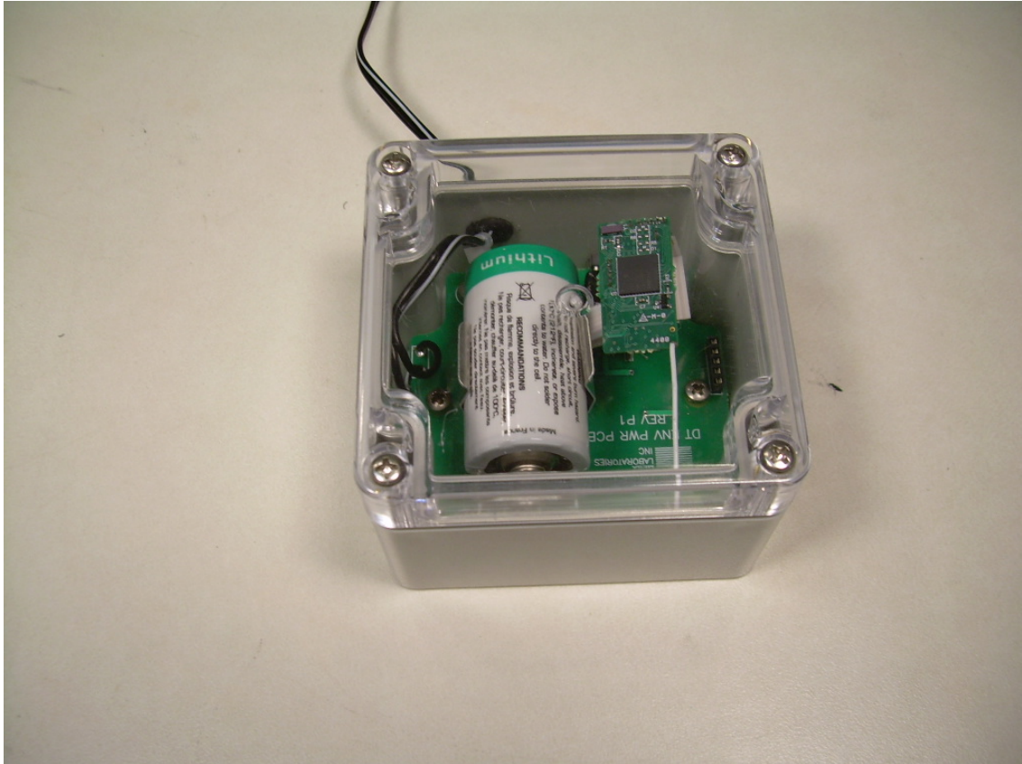
Front View of the DTENV-R
