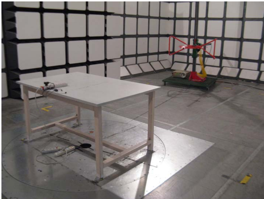
Radiated Emissions - Rear View (Charging)
