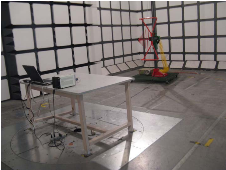
Transmitting Mode: Radiated Emissions - Rear View (30 – 1000 MHz)
