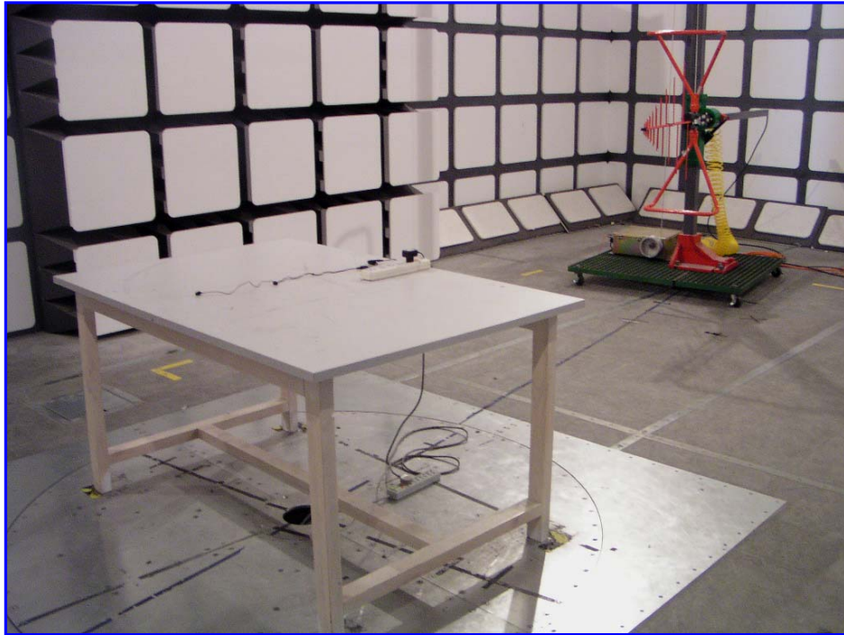
Charging Mode: Radiated Emissions - Front View
