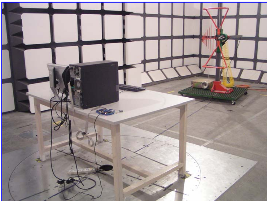
Transmitting Mode: Radiated Emissions - Front View (30-1000MHz)
