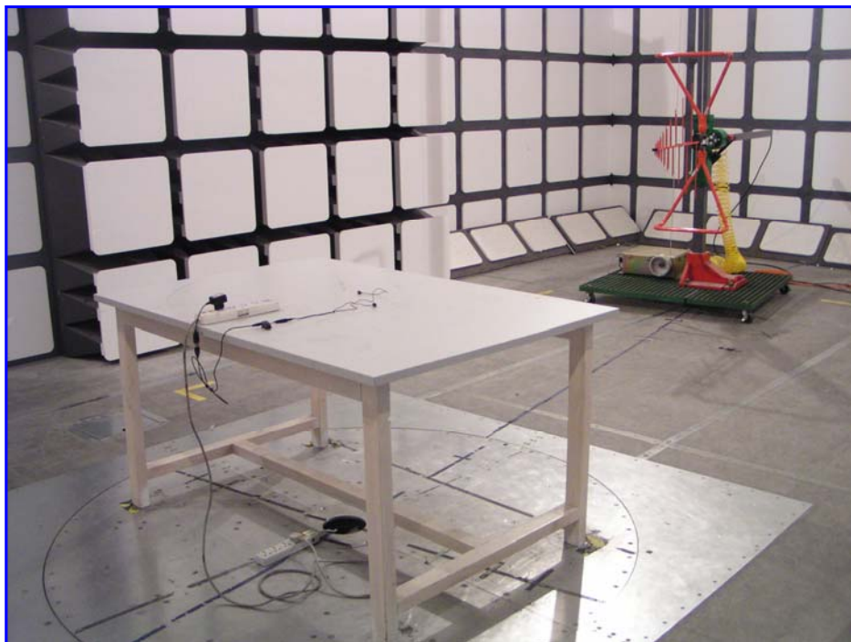
Charging Mode: Radiated Emissions - Rear View
