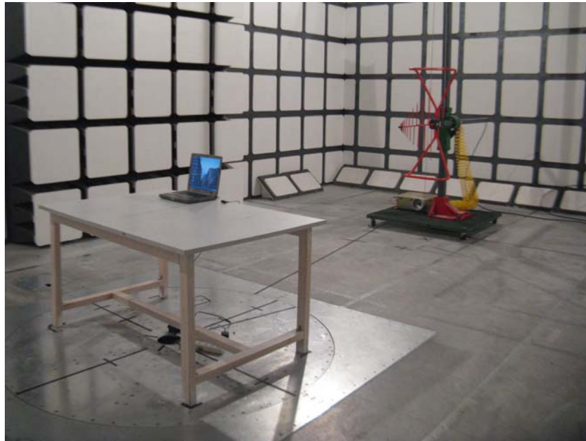
Radiated Emissions - Front View (PC Charging)
