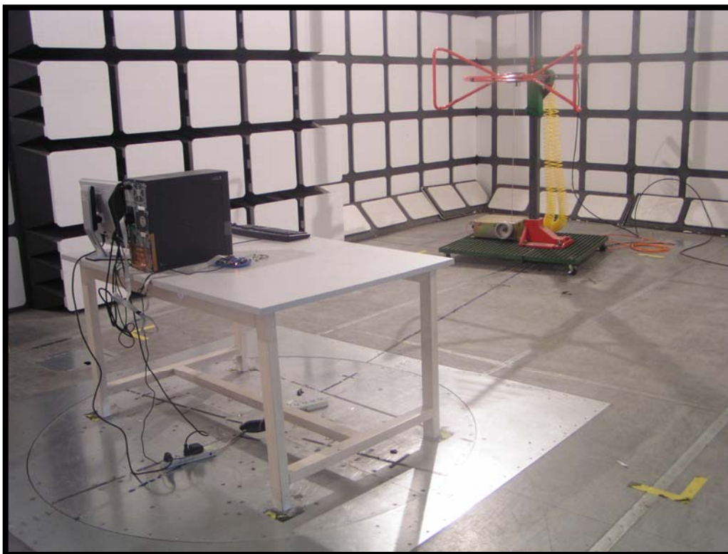
Radiated Emission (30 to 1000 MHz) - Rear View
