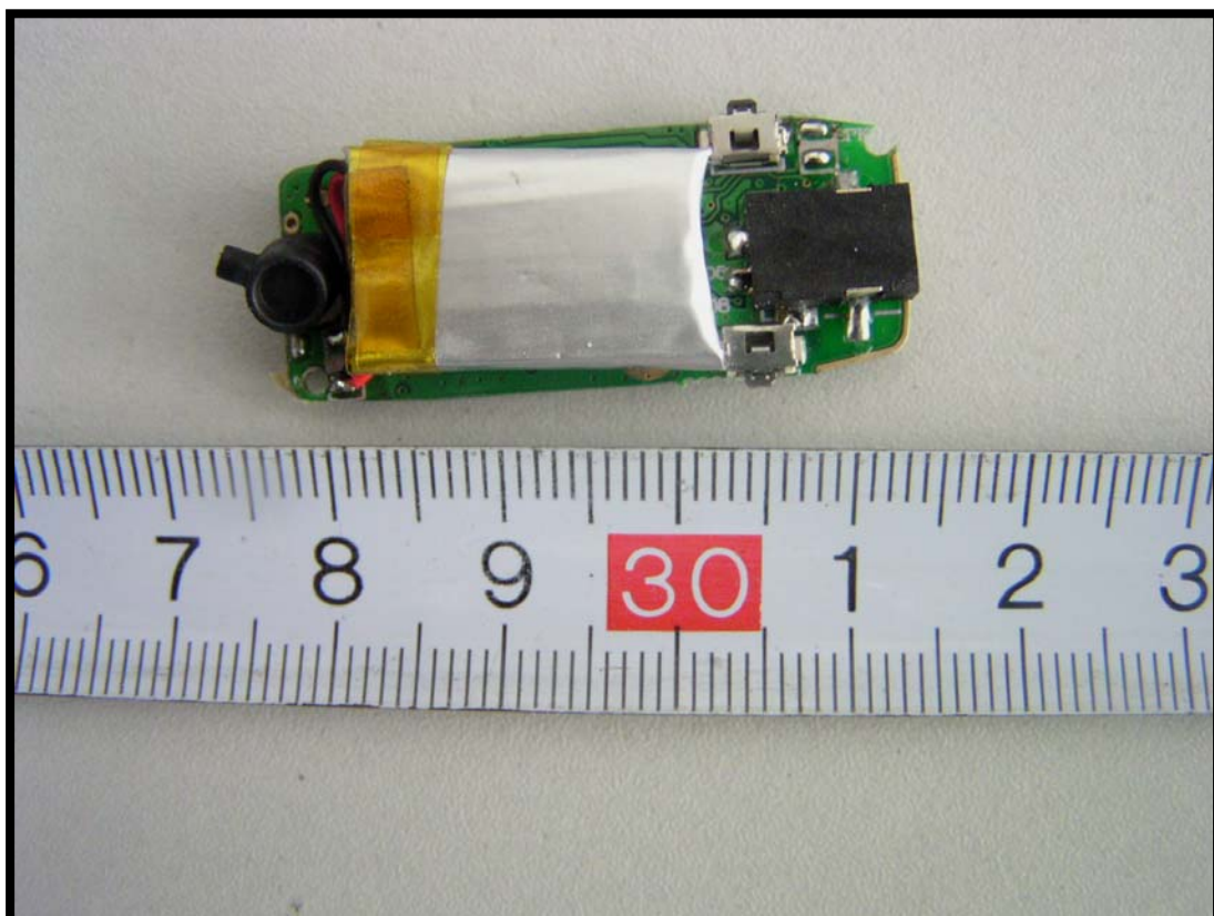
EUT-Main board and Battery View
