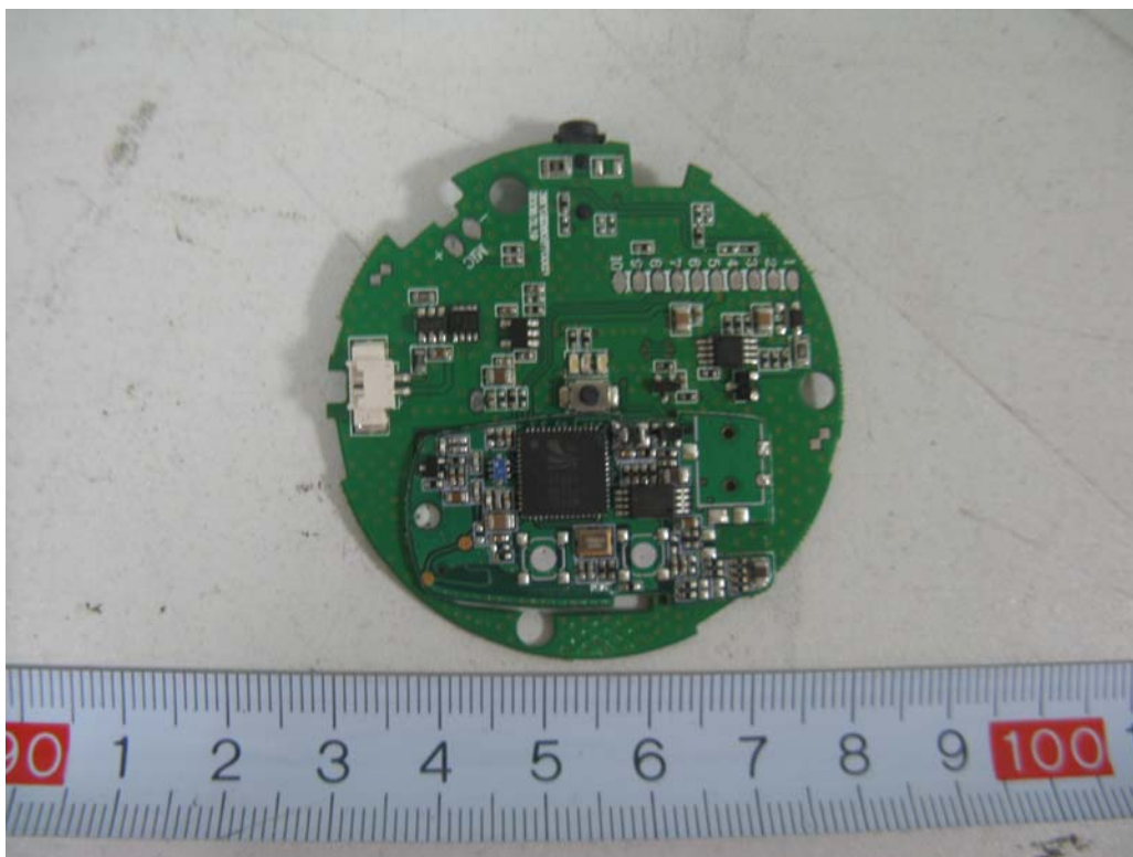
EUT - Bluetooth Board Top Components View
