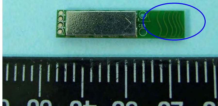
Bluetooth Antenna
