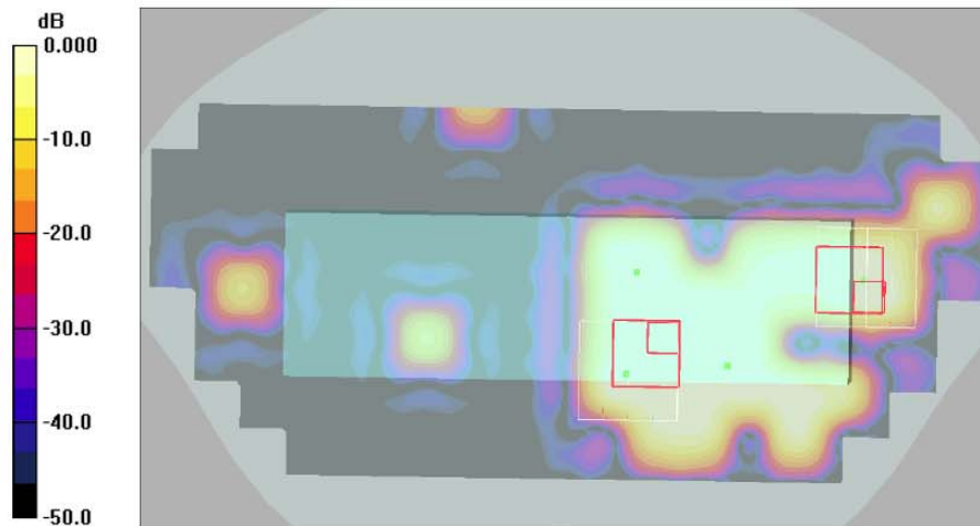
0 dB = 0.006mW/g
