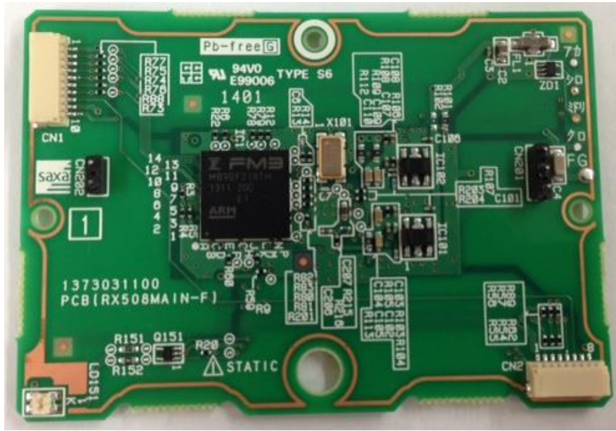
(1)The Upper-Side of Main Substrate
