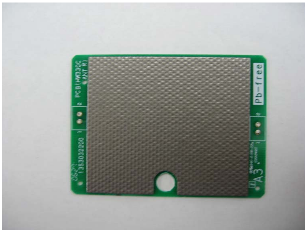
Antenna back
