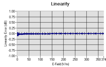
Linearity: \pm 1.95\% ( \pm 0.09\text{dB} )
