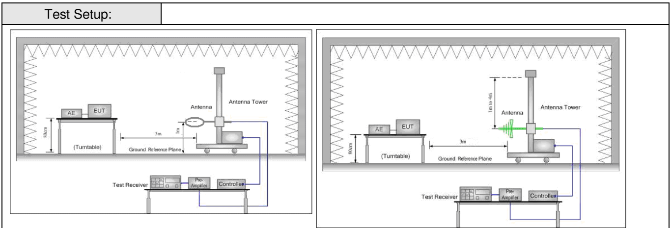
Figure 1. Below 30MHz
