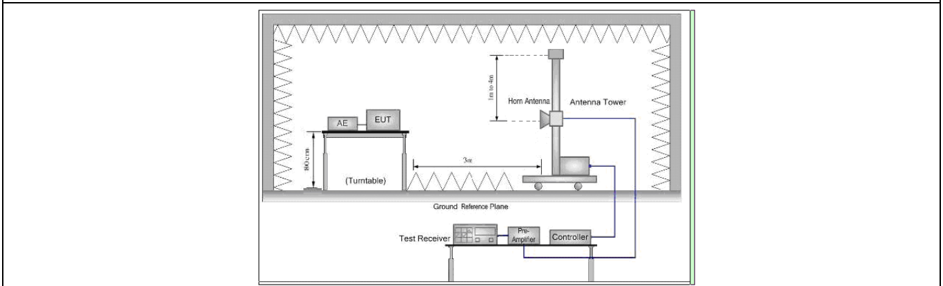
Figure 3. Above 1 GHz
