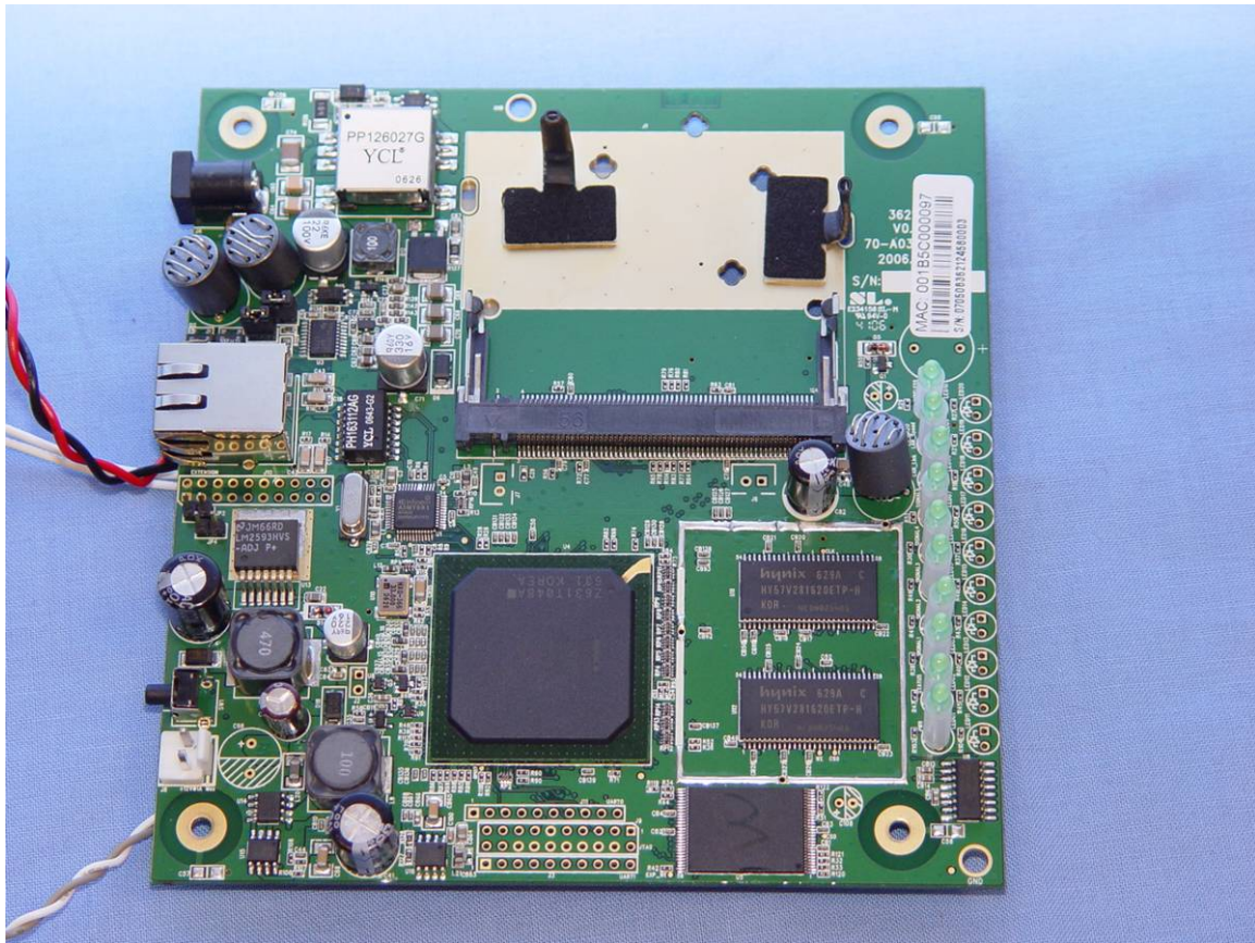
Motherboard Front
