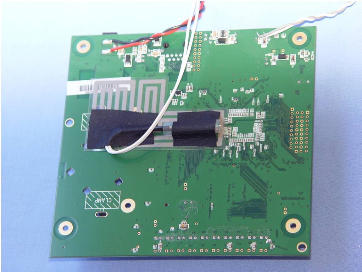
Motherboard rear
