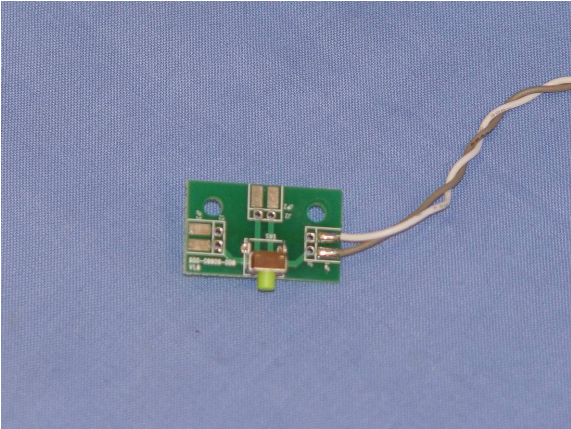
Reset Switch Front
