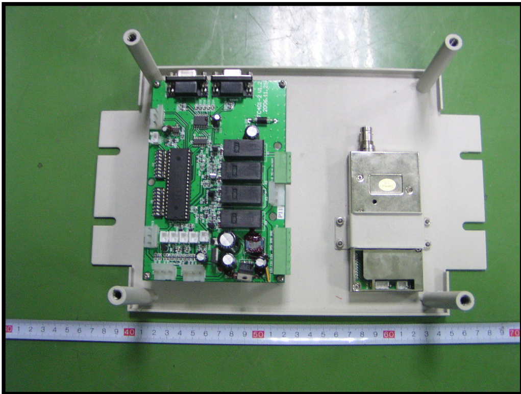
EUT – Uncovered View (3)
