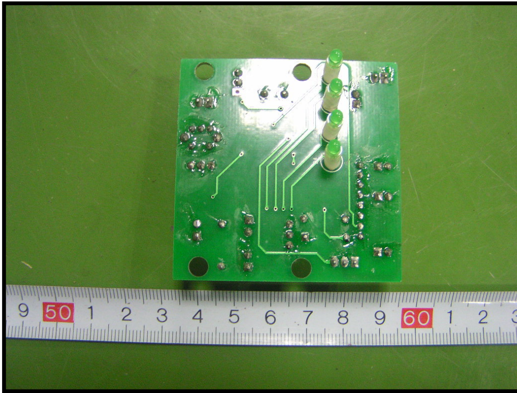
EUT – Board 2 Circuit View
