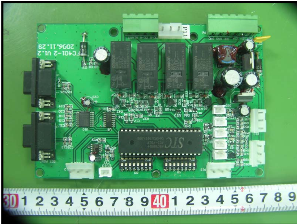
EUT – Board 3 Component View
