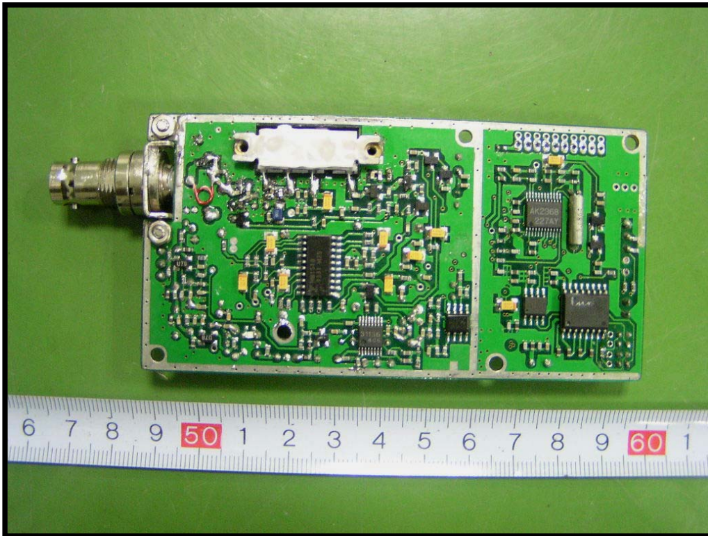
EUT – Board 1 Component Bottom View
