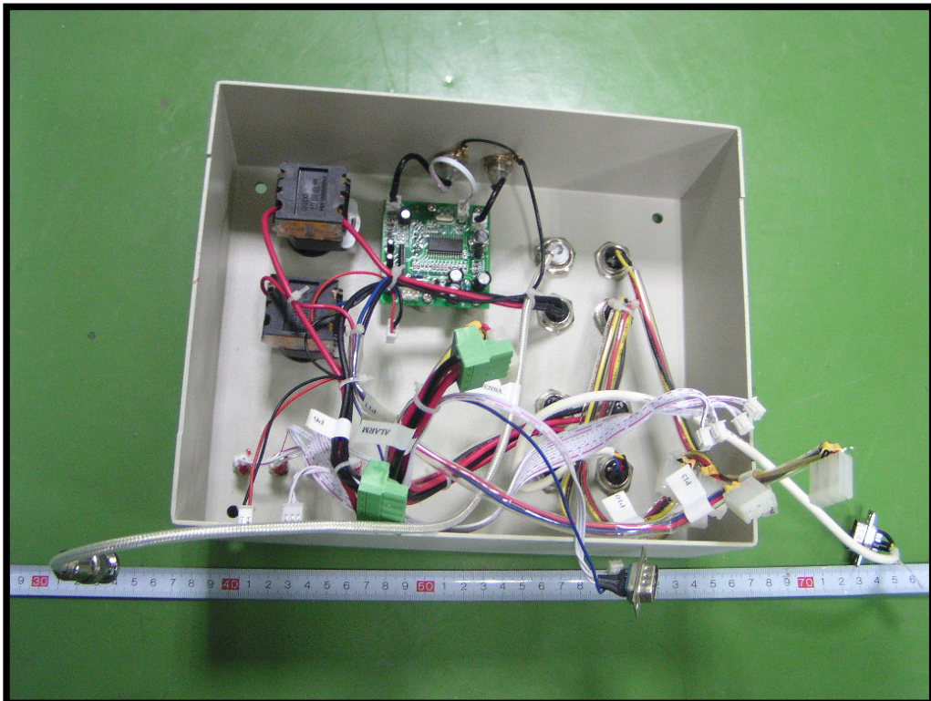
EUT – Uncovered View (2)
