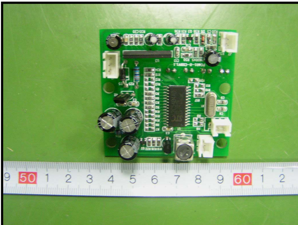
EUT – Board 2 Component View
