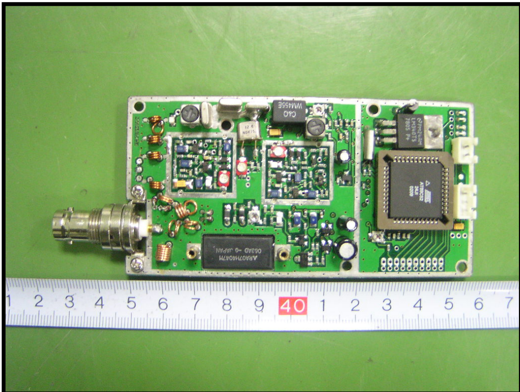
EUT – Board 1 Component Top View
