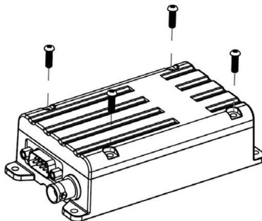
Fig. 19-Upper Cover Removal
