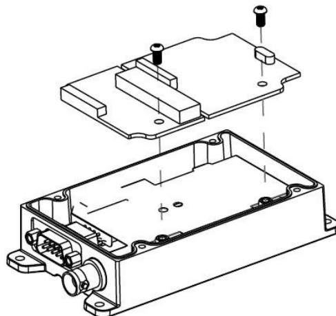
Fig. 20-Power board & Modem board Assembly Removal
