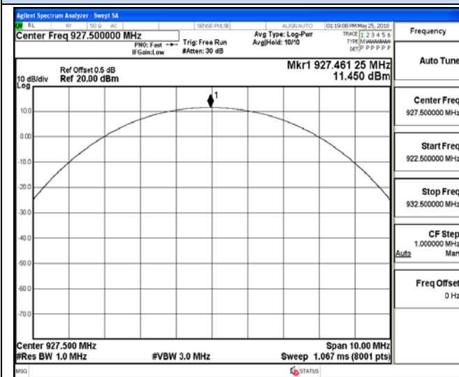
Channel 10 / 927.5 MHz
