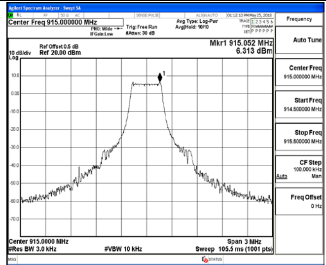
Channel 05 / 915 MHz
