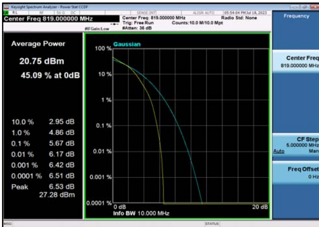
FDD26_Part 90_LowRange_10MHz_819_fullIRB_Q16
