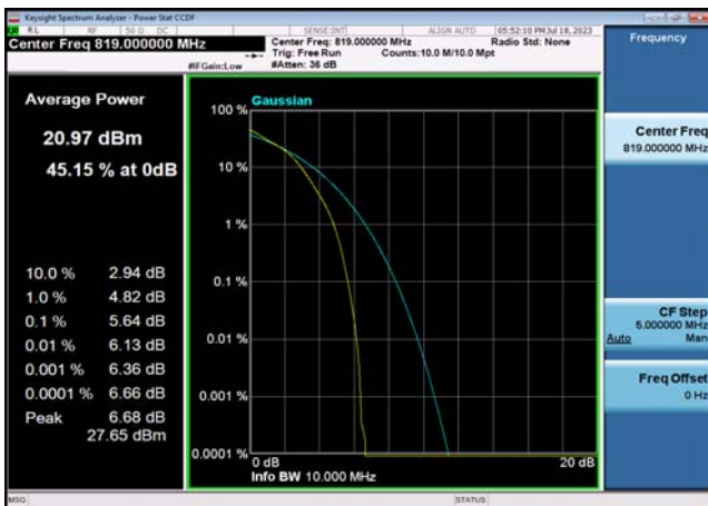
FDD26_Part 90_MidRange_10MHz_819_fullIRB_Q16
