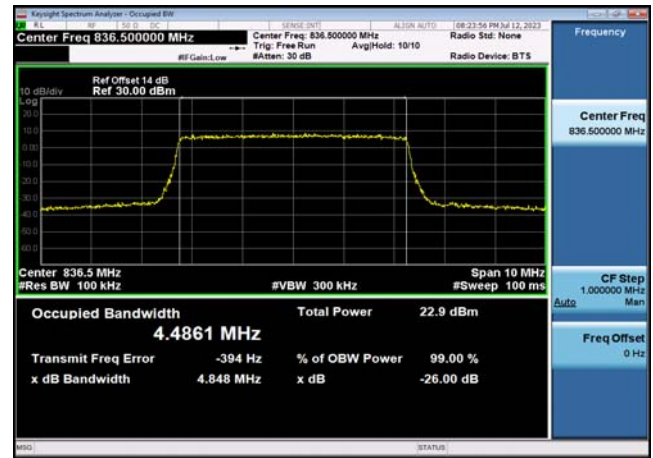
FDD26_(Part 22&RSS-132) _MidRange_10_836.5_Q16
