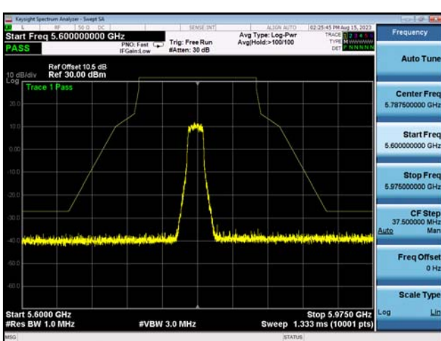
U-NII-3 ,Plot 1,Band Edge-802.11a(20 Hz),5785MHz,Ant1
