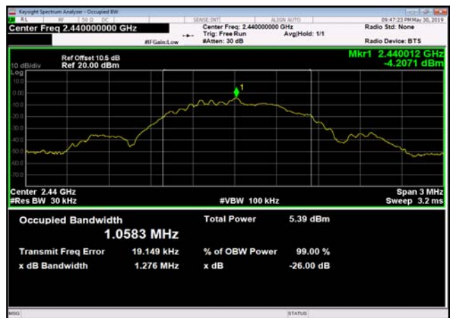
99% Bandwidth: 2440MHz
